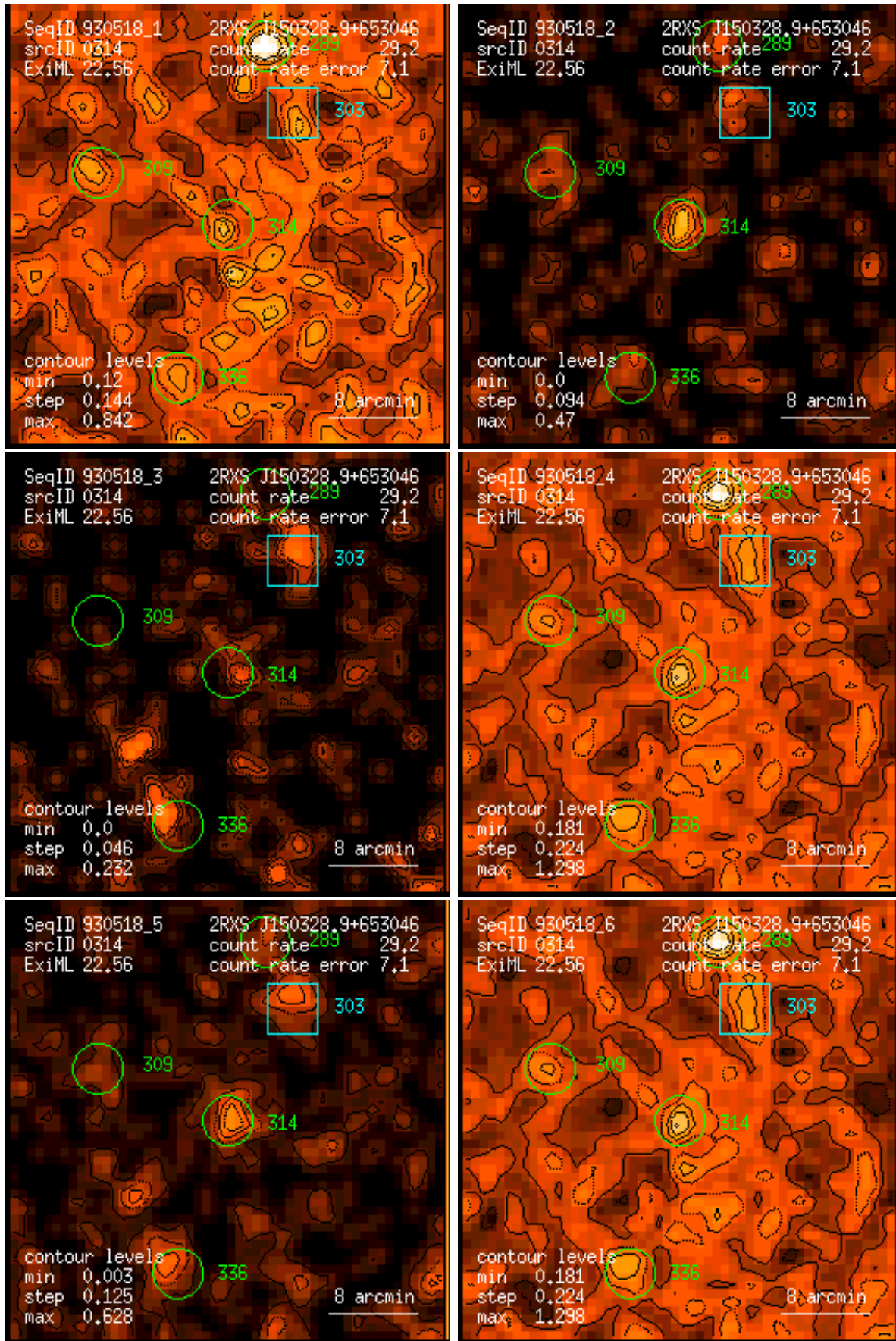
Figure 314: RASS 930518: detection 0314: band rate images, Gaussian filter: (1) PSPC channels 11 – 41, (2) 52 – 90, (3) 91 – 201, (4) 11 – 235, (5) 52 – 201, (6) 11 – 201. Broad band rates in counts/ks. Band rate contour levels in counts/ks/arcmin 2 .
