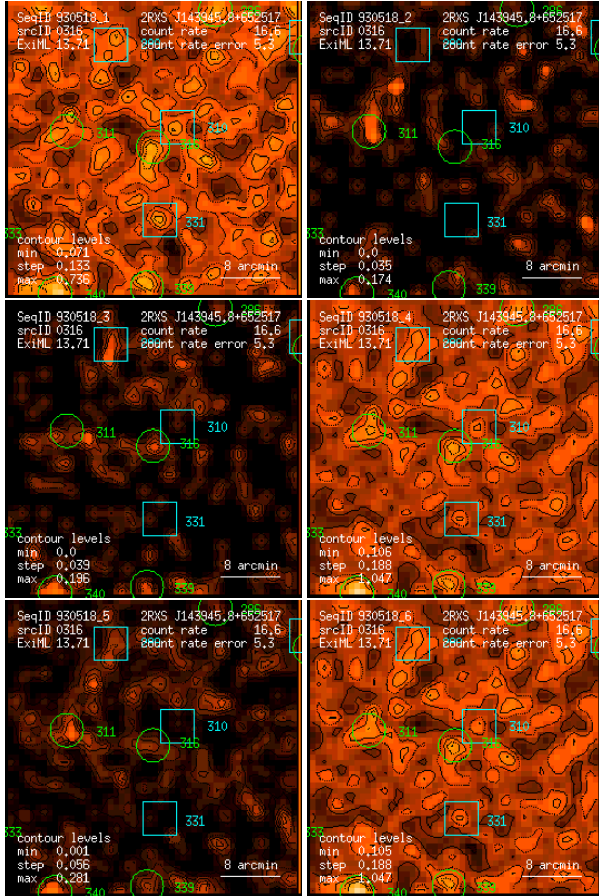
Figure 316: RASS 930518: detection 0316: band rate images, Gaussian filter: (1) PSPC channels 11 – 41, (2) 52 – 90, (3) 91 – 201, (4) 11 – 235, (5) 52 – 201, (6) 11 – 201. Broad band rates in counts/ks. Band rate contour levels in counts/ks/arcmin 2 .
