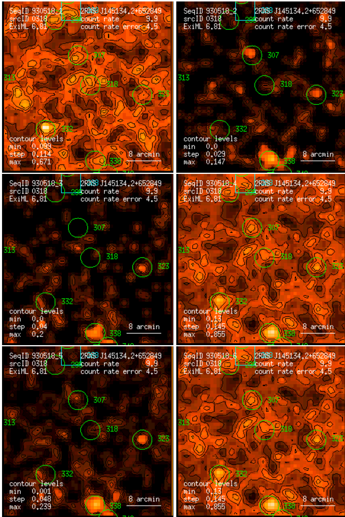
Figure 318: RASS 930518: detection 0318: band rate images, Gaussian filter: (1) PSPC channels 11 – 41, (2) 52 – 90, (3) 91 – 201, (4) 11 – 235, (5) 52 – 201, (6) 11 – 201. Broad band rates in counts/ks. Band rate contour levels in counts/ks/arcmin 2 .
