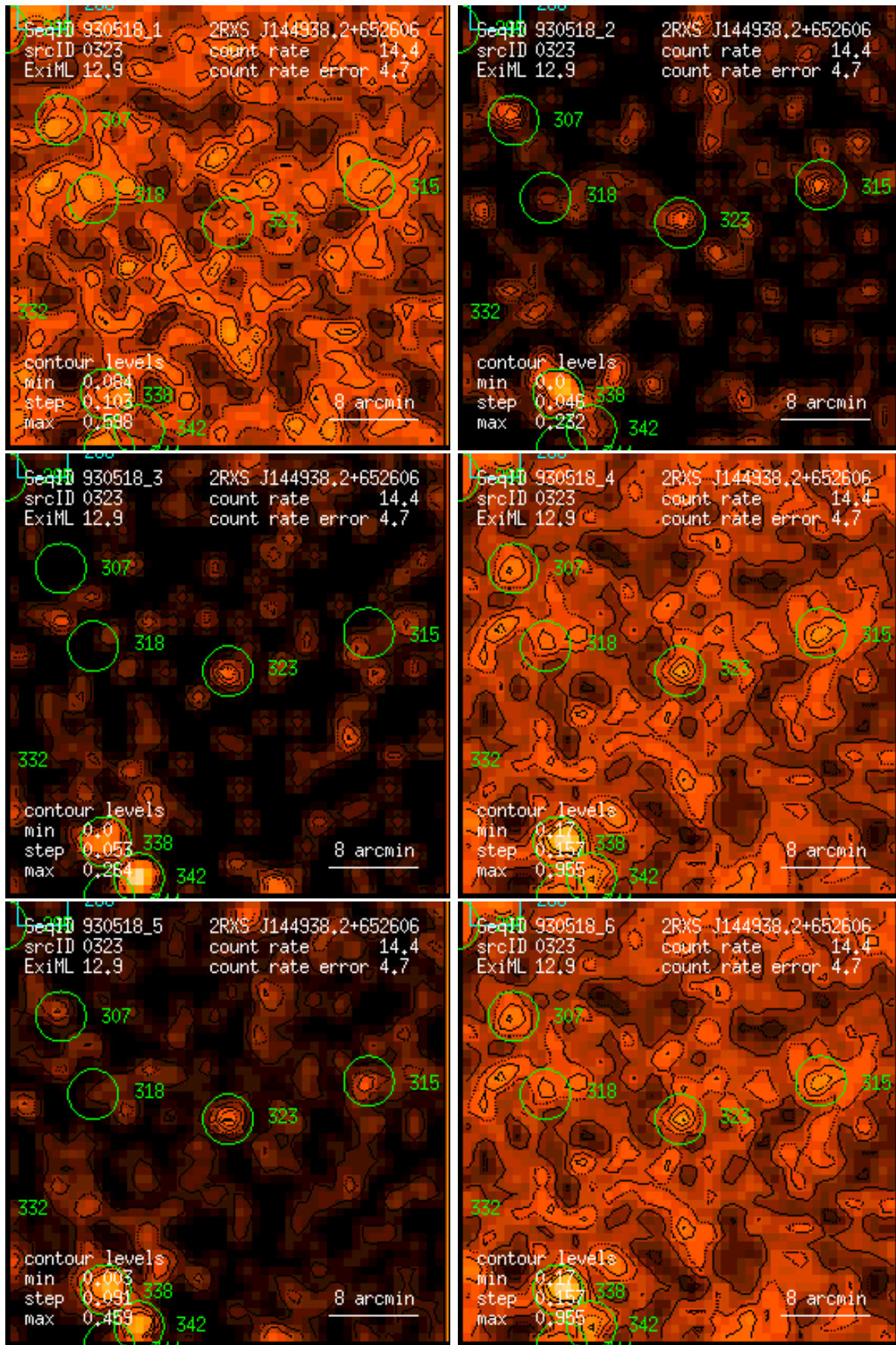
Figure 323: RASS 930518: detection 0323: band rate images, Gaussian filter: (1) PSPC channels 11 – 41, (2) 52 – 90, (3) 91 – 201, (4) 11 – 235, (5) 52 – 201, (6) 11 – 201. Broad band rates in counts/ks. Band rate contour levels in counts/ks/arcmin 2 .
