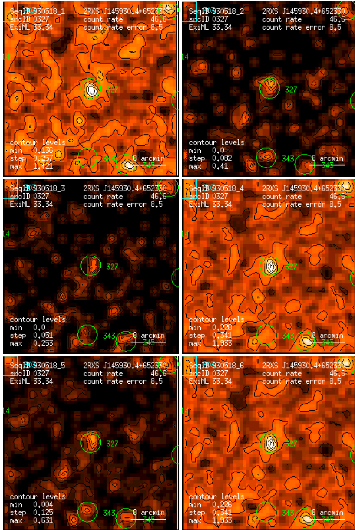
Figure 327: RASS 930518: detection 0327: band rate images, Gaussian filter: (1) PSPC channels 11 – 41, (2) 52 – 90, (3) 91 – 201, (4) 11 – 235, (5) 52 – 201, (6) 11 – 201. Broad band rates in counts/ks. Band rate contour levels in counts/ks/arcmin 2 .
