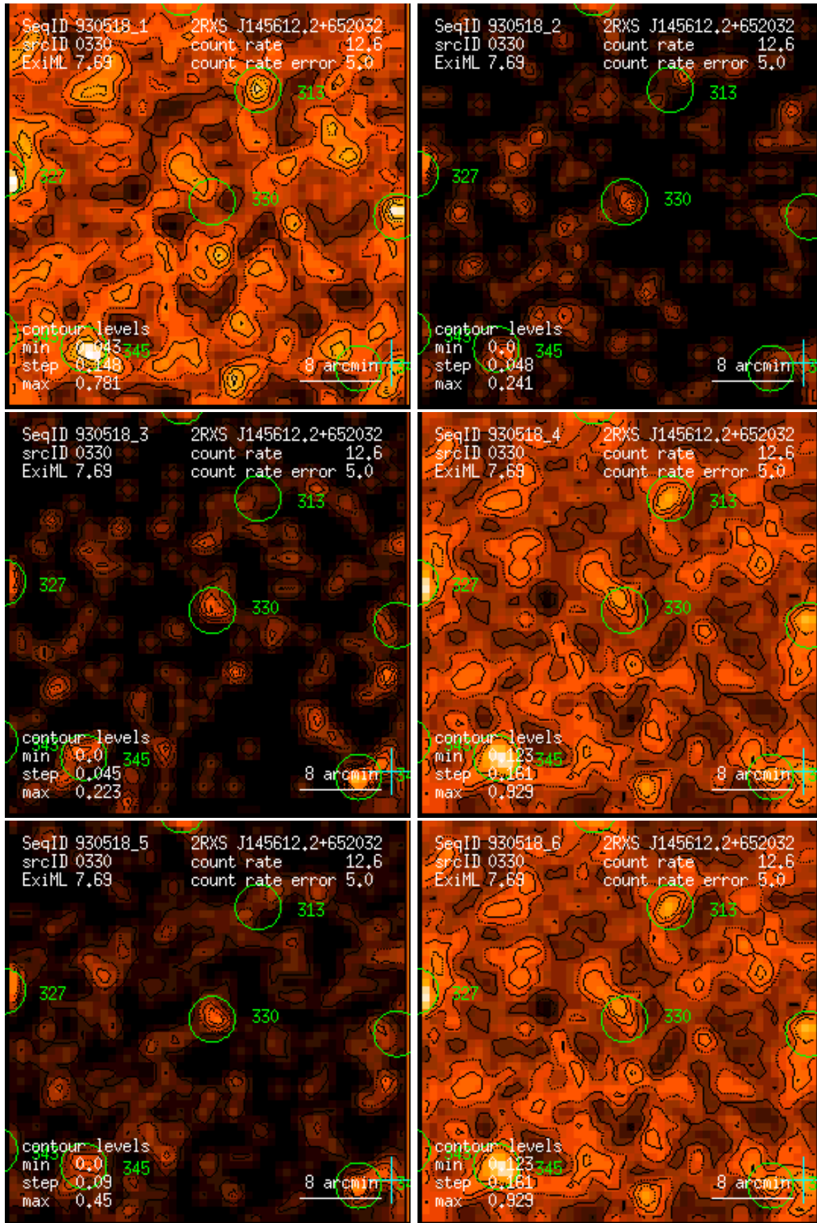
Figure 330: RASS 930518: detection 0330: band rate images, Gaussian filter: (1) PSPC channels 11 – 41, (2) 52 – 90, (3) 91 – 201, (4) 11 – 235, (5) 52 – 201, (6) 11 – 201. Broad band rates in counts/ks. Band rate contour levels in counts/ks/arcmin 2 .
