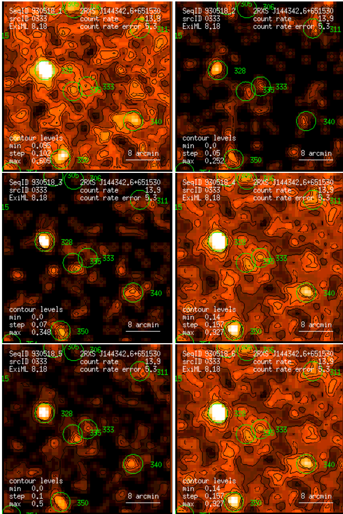
Figure 333: RASS 930518: detection 0333: band rate images, Gaussian filter: (1) PSPC channels 11 – 41, (2) 52 – 90, (3) 91 – 201, (4) 11 – 235, (5) 52 – 201, (6) 11 – 201. Broad band rates in counts/ks. Band rate contour levels in counts/ks/arcmin 2 .
