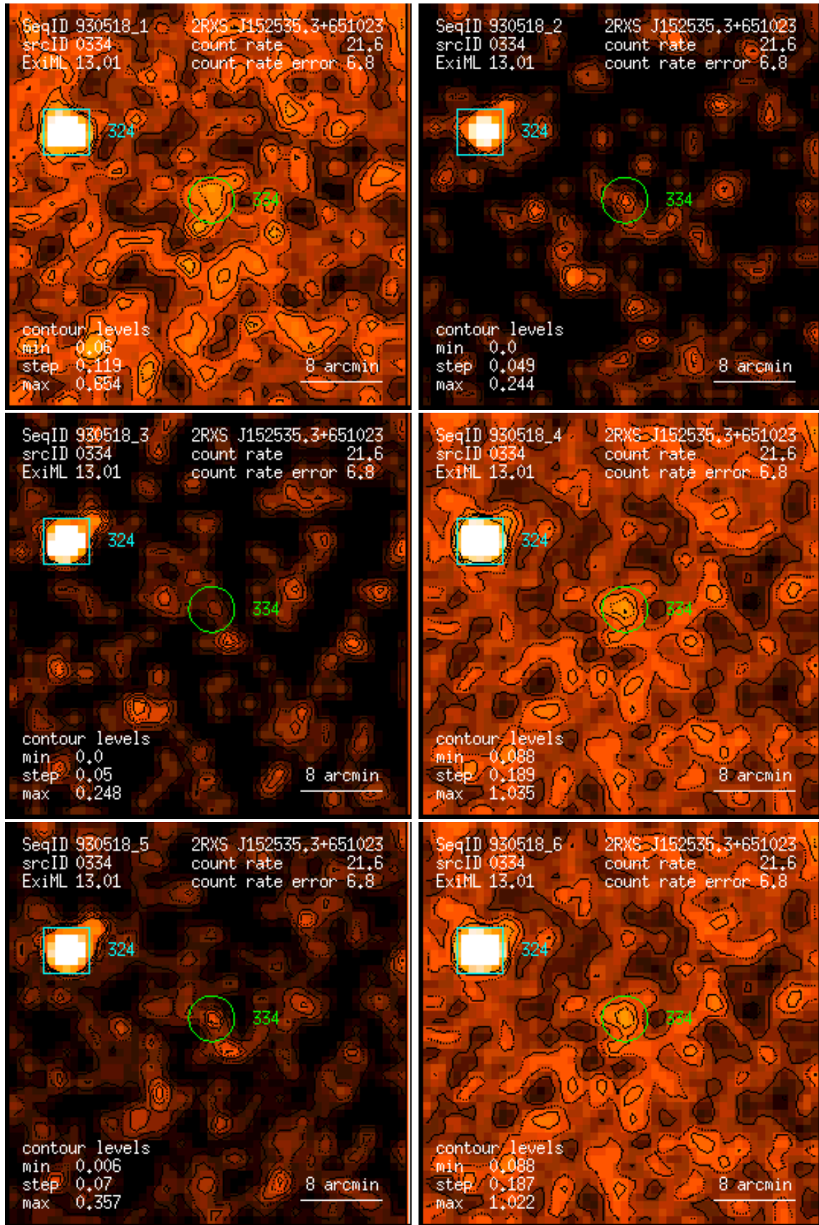
Figure 334: RASS 930518: detection 0334: band rate images, Gaussian filter: (1) PSPC channels 11 – 41, (2) 52 – 90, (3) 91 – 201, (4) 11 – 235, (5) 52 – 201, (6) 11 – 201. Broad band rates in counts/ks. Band rate contour levels in counts/ks/arcmin 2 .
