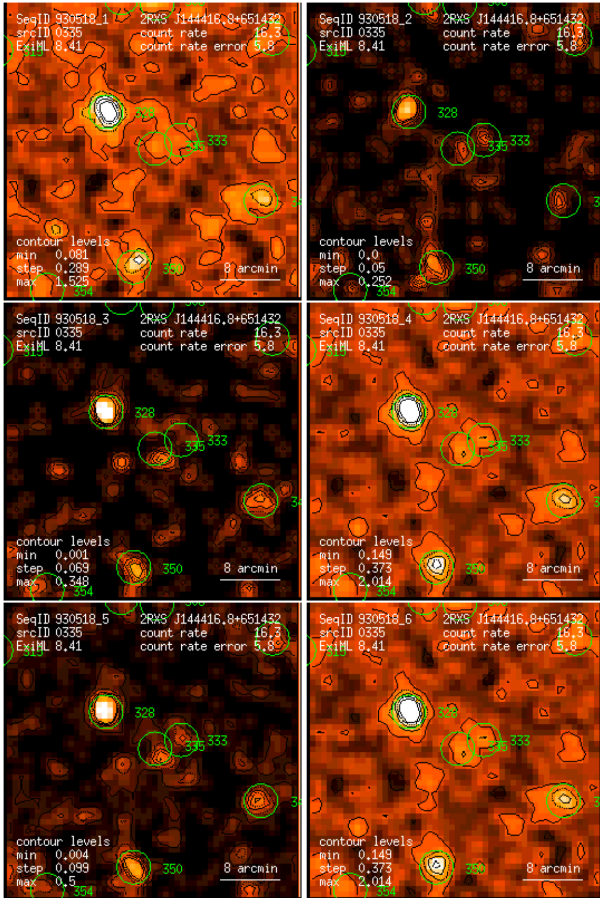
Figure 335: RASS 930518: detection 0335: band rate images, Gaussian filter: (1) PSPC channels 11 – 41, (2) 52 – 90, (3) 91 – 201, (4) 11 – 235, (5) 52 – 201, (6) 11 – 201. Broad band rates in counts/ks. Band rate contour levels in counts/ks/arcmin 2 .
