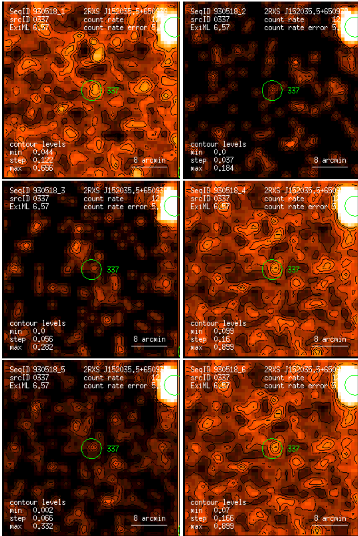
Figure 337: RASS 930518: detection 0337: band rate images, Gaussian filter: (1) PSPC channels 11 – 41, (2) 52 – 90, (3) 91 – 201, (4) 11 – 235, (5) 52 – 201, (6) 11 – 201. Broad band rates in counts/ks. Band rate contour levels in counts/ks/arcmin 2 .
