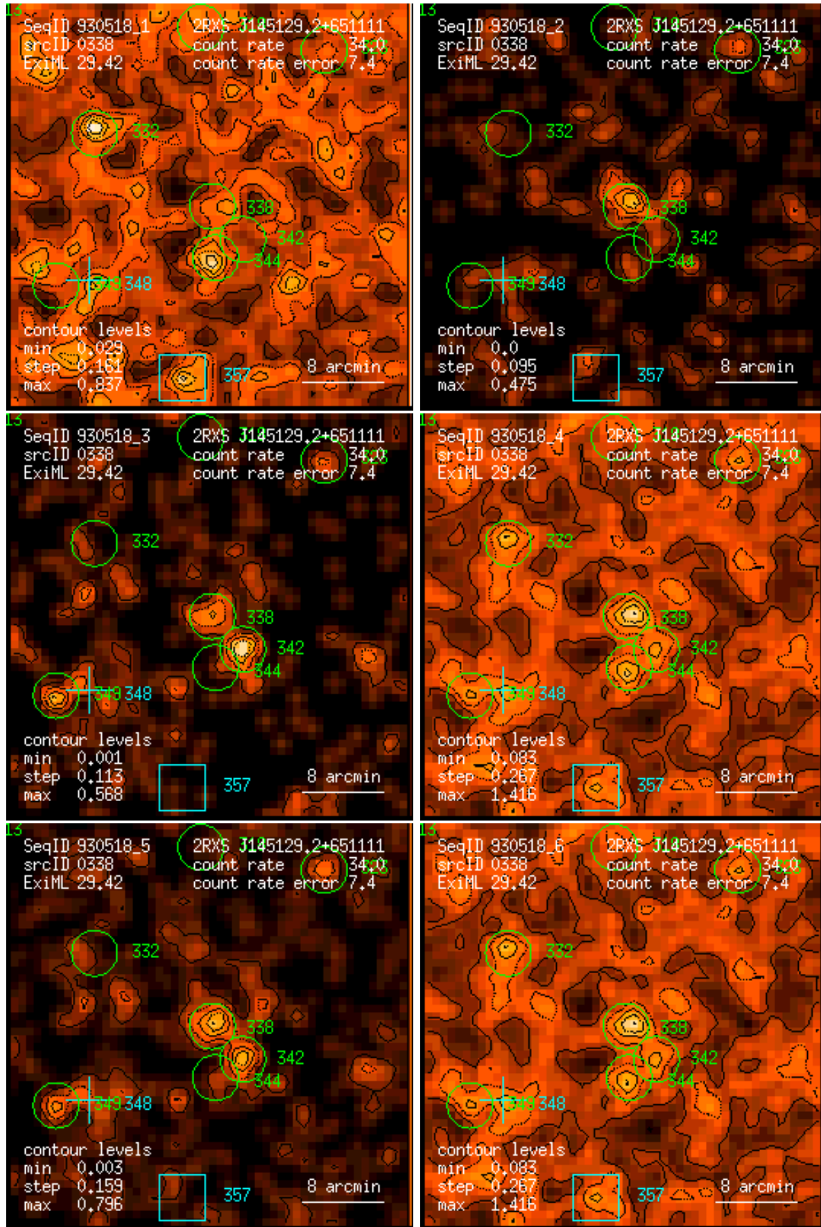
Figure 338: RASS 930518: detection 0338: band rate images, Gaussian filter: (1) PSPC channels 11 – 41, (2) 52 – 90, (3) 91 – 201, (4) 11 – 235, (5) 52 – 201, (6) 11 – 201. Broad band rates in counts/ks. Band rate contour levels in counts/ks/arcmin 2 .
