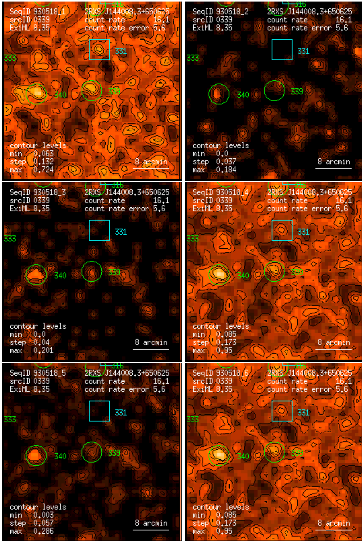
Figure 339: RASS 930518: detection 0339: band rate images, Gaussian filter: (1) PSPC channels 11 – 41, (2) 52 – 90, (3) 91 – 201, (4) 11 – 235, (5) 52 – 201, (6) 11 – 201. Broad band rates in counts/ks. Band rate contour levels in counts/ks/arcmin 2 .
