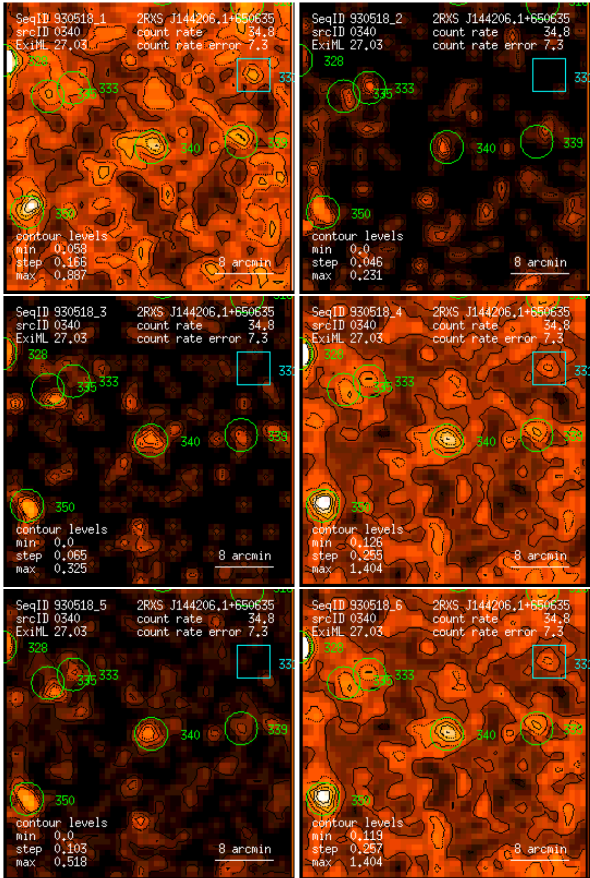
Figure 340: RASS 930518: detection 0340: band rate images, Gaussian filter: (1) PSPC channels 11 – 41, (2) 52 – 90, (3) 91 – 201, (4) 11 – 235, (5) 52 – 201, (6) 11 – 201. Broad band rates in counts/ks. Band rate contour levels in counts/ks/arcmin 2 .
