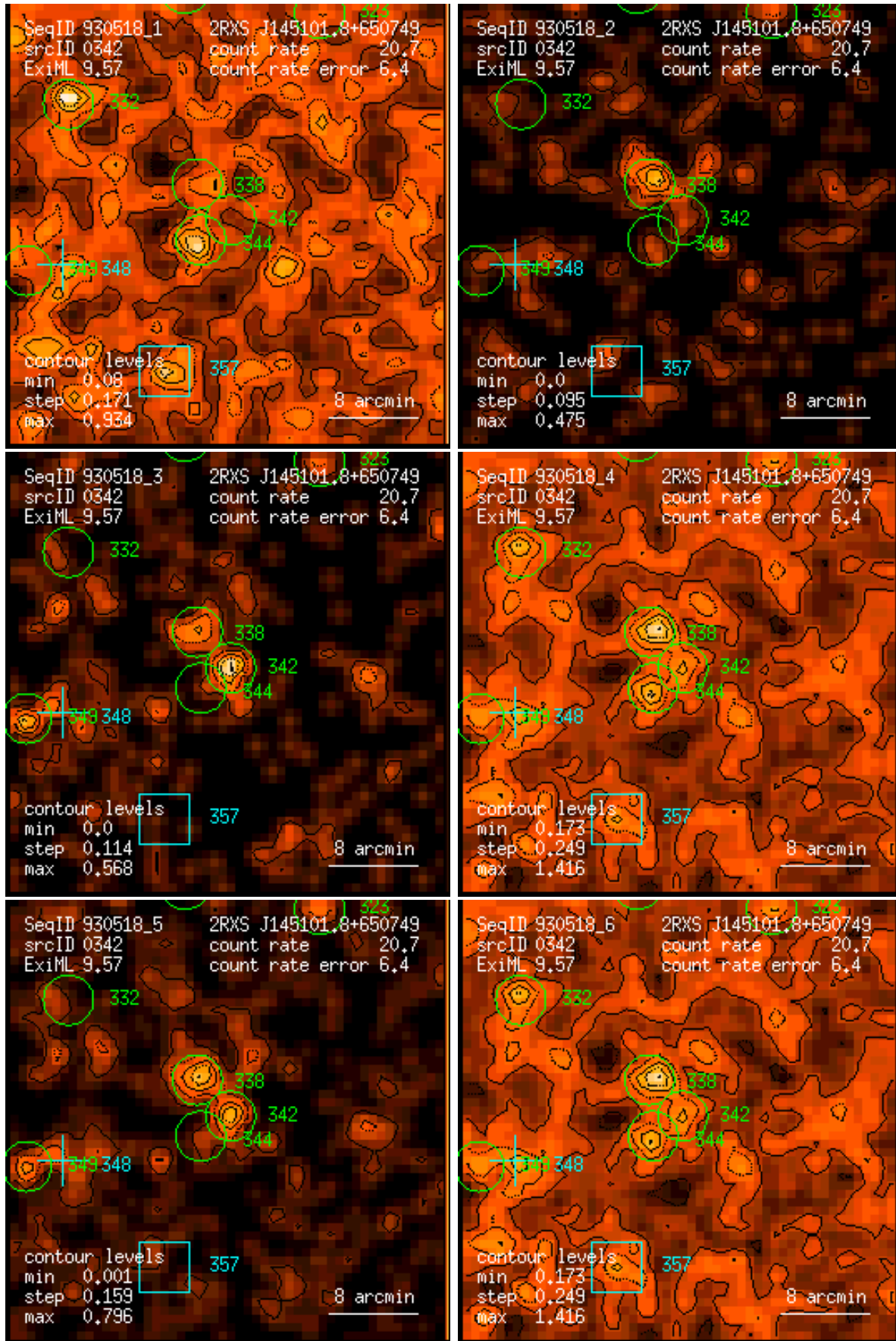
Figure 342: RASS 930518: detection 0342: band rate images, Gaussian filter: (1) PSPC channels 11 – 41, (2) 52 – 90, (3) 91 – 201, (4) 11 – 235, (5) 52 – 201, (6) 11 – 201. Broad band rates in counts/ks. Band rate contour levels in counts/ks/arcmin 2 .
