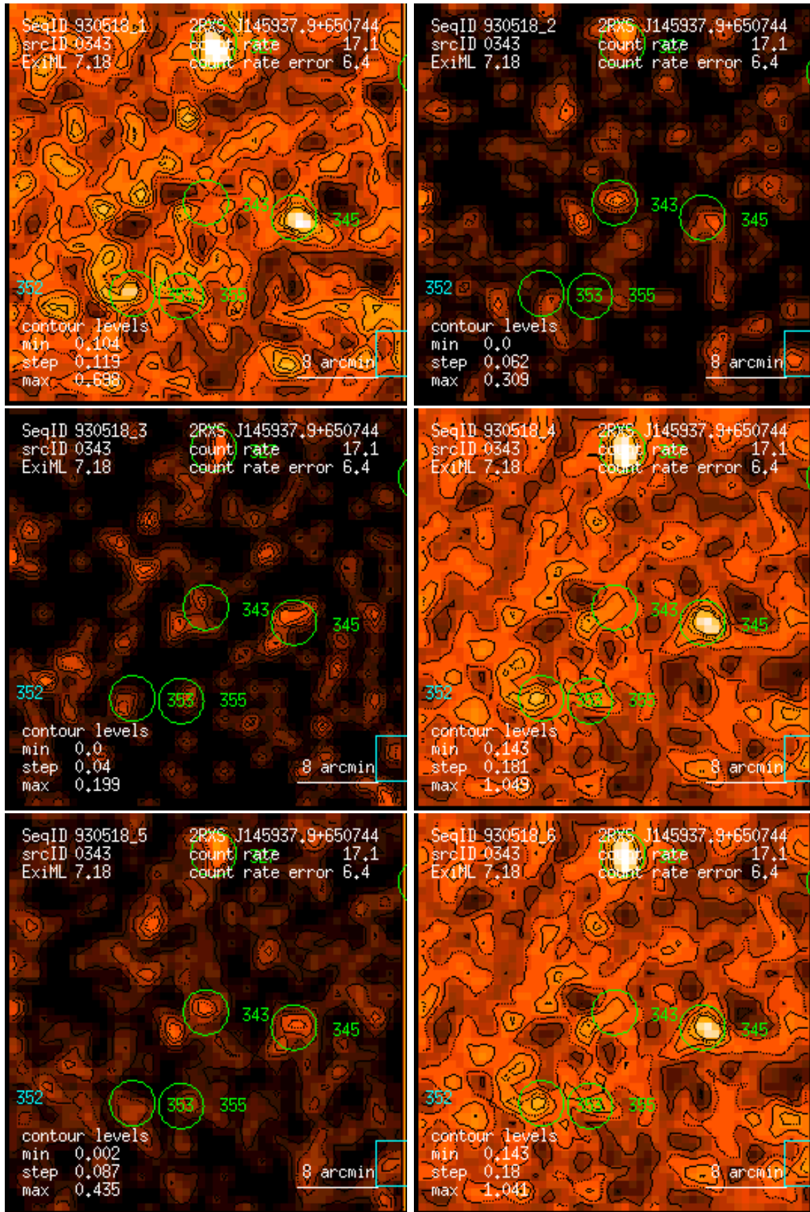
Figure 343: RASS 930518: detection 0343: band rate images, Gaussian filter: (1) PSPC channels 11 – 41, (2) 52 – 90, (3) 91 – 201, (4) 11 – 235, (5) 52 – 201, (6) 11 – 201. Broad band rates in counts/ks. Band rate contour levels in counts/ks/arcmin 2 .
