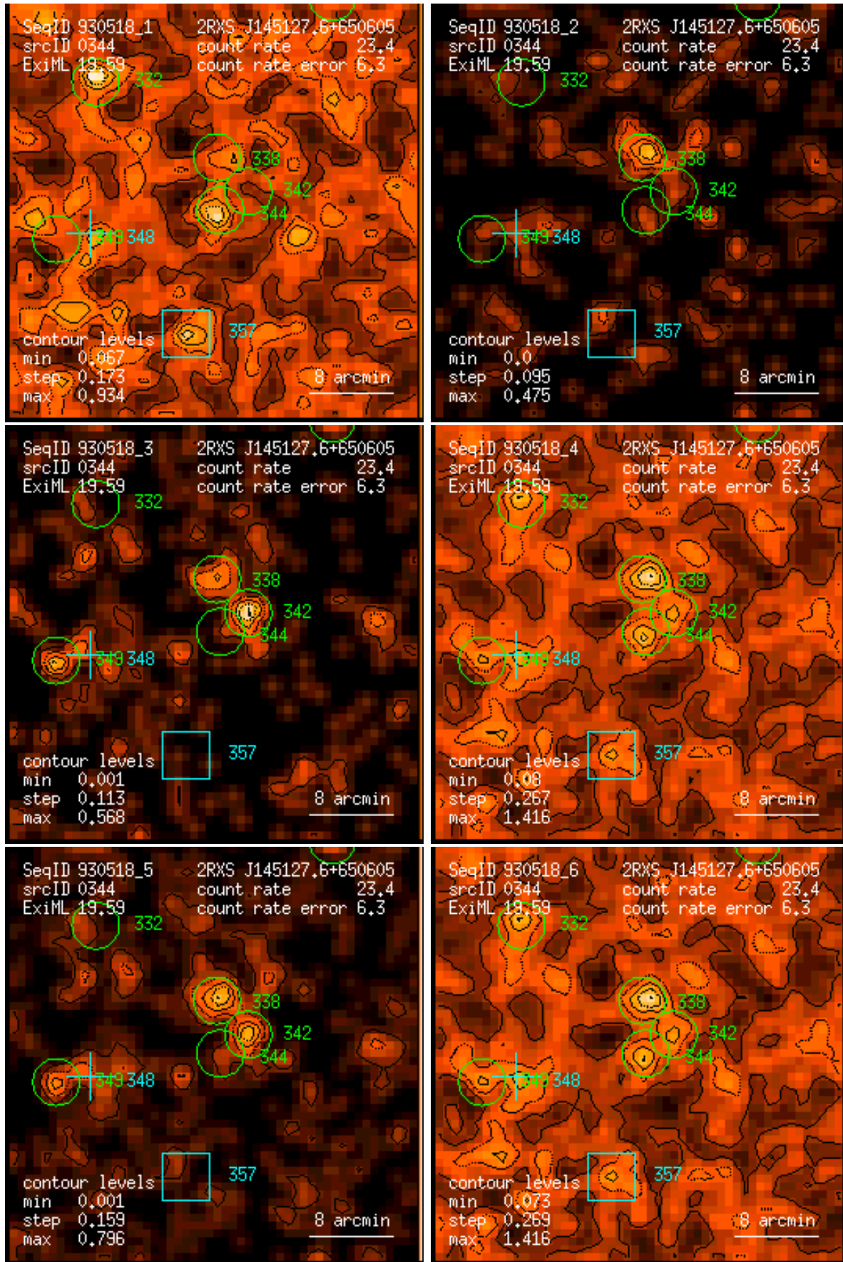
Figure 344: RASS 930518: detection 0344: band rate images, Gaussian filter: (1) PSPC channels 11 – 41, (2) 52 – 90, (3) 91 – 201, (4) 11 – 235, (5) 52 – 201, (6) 11 – 201. Broad band rates in counts/ks. Band rate contour levels in counts/ks/arcmin 2 .
