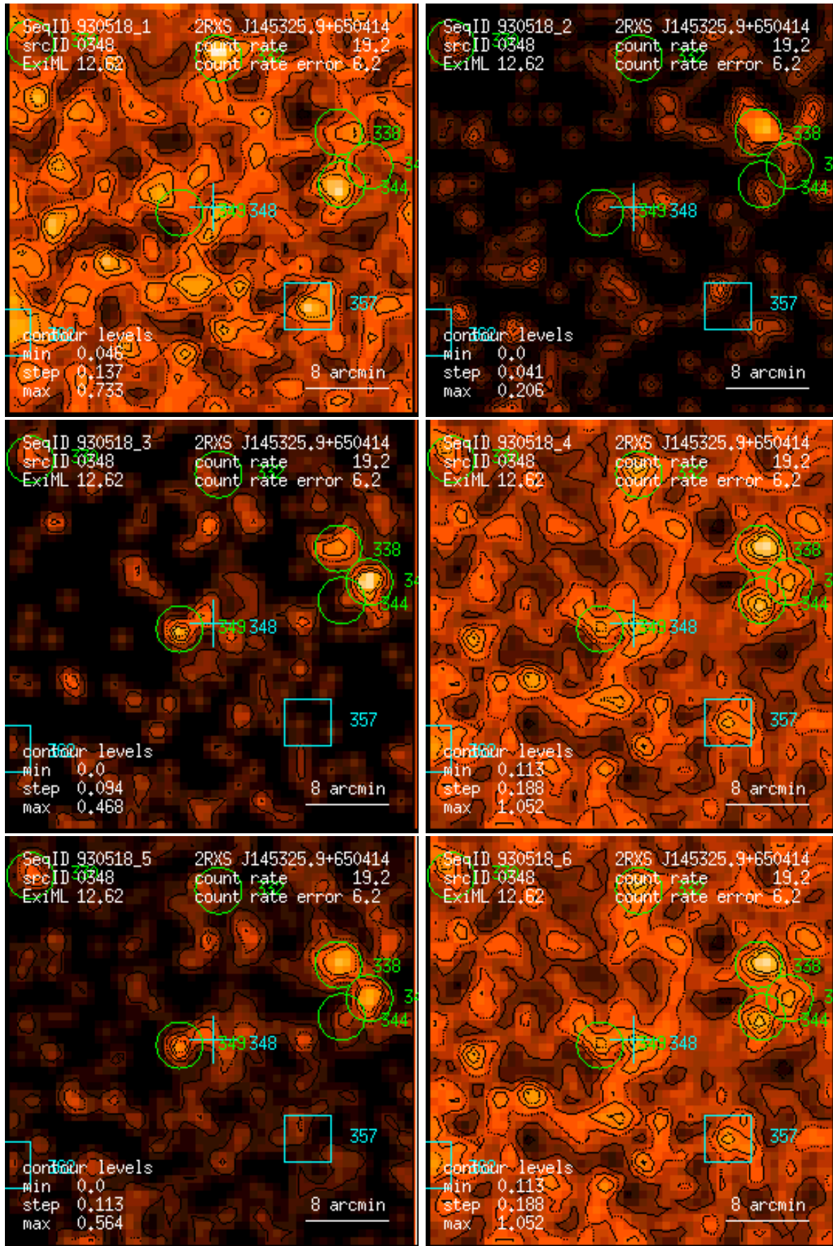
Figure 348: RASS 930518: detection 0348: band rate images, Gaussian filter: (1) PSPC channels 11 – 41, (2) 52 – 90, (3) 91 – 201, (4) 11 – 235, (5) 52 – 201, (6) 11 – 201. Broad band rates in counts/ks. Band rate contour levels in counts/ks/arcmin 2 .
