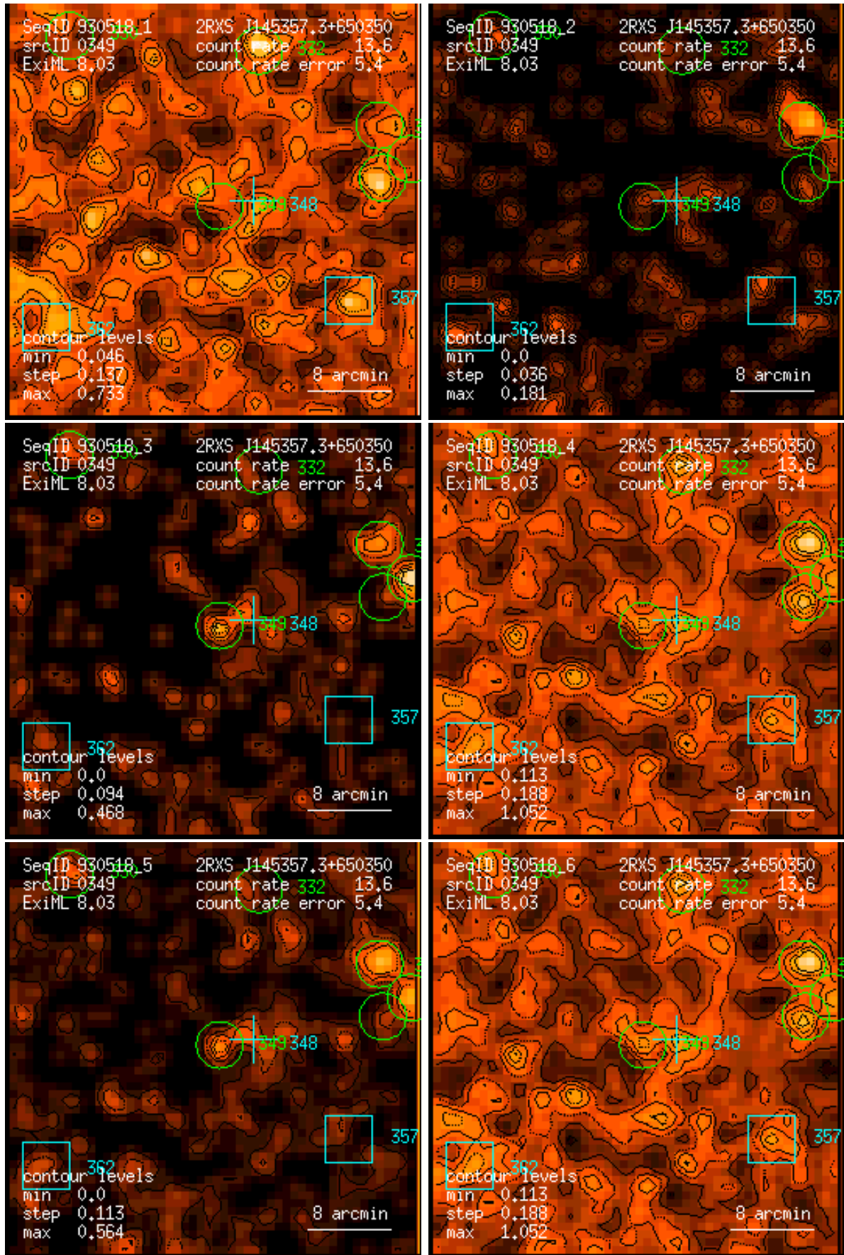
Figure 349: RASS 930518: detection 0349: band rate images, Gaussian filter: (1) PSPC channels 11 – 41, (2) 52 – 90, (3) 91 – 201, (4) 11 – 235, (5) 52 – 201, (6) 11 – 201. Broad band rates in counts/ks. Band rate contour levels in counts/ks/arcmin 2 .
