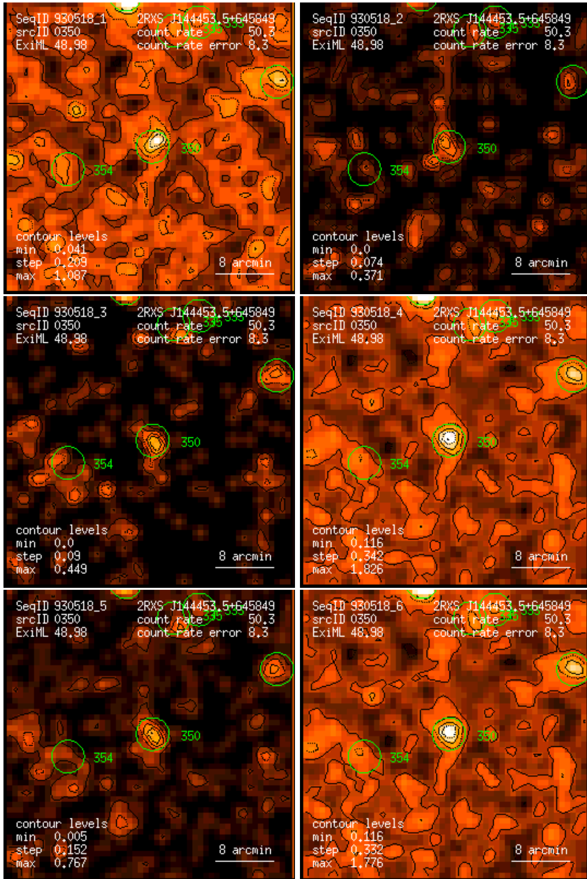
Figure 350: RASS 930518: detection 0350: band rate images, Gaussian filter: (1) PSPC channels 11 – 41, (2) 52 – 90, (3) 91 – 201, (4) 11 – 235, (5) 52 – 201, (6) 11 – 201. Broad band rates in counts/ks. Band rate contour levels in counts/ks/arcmin 2 .
