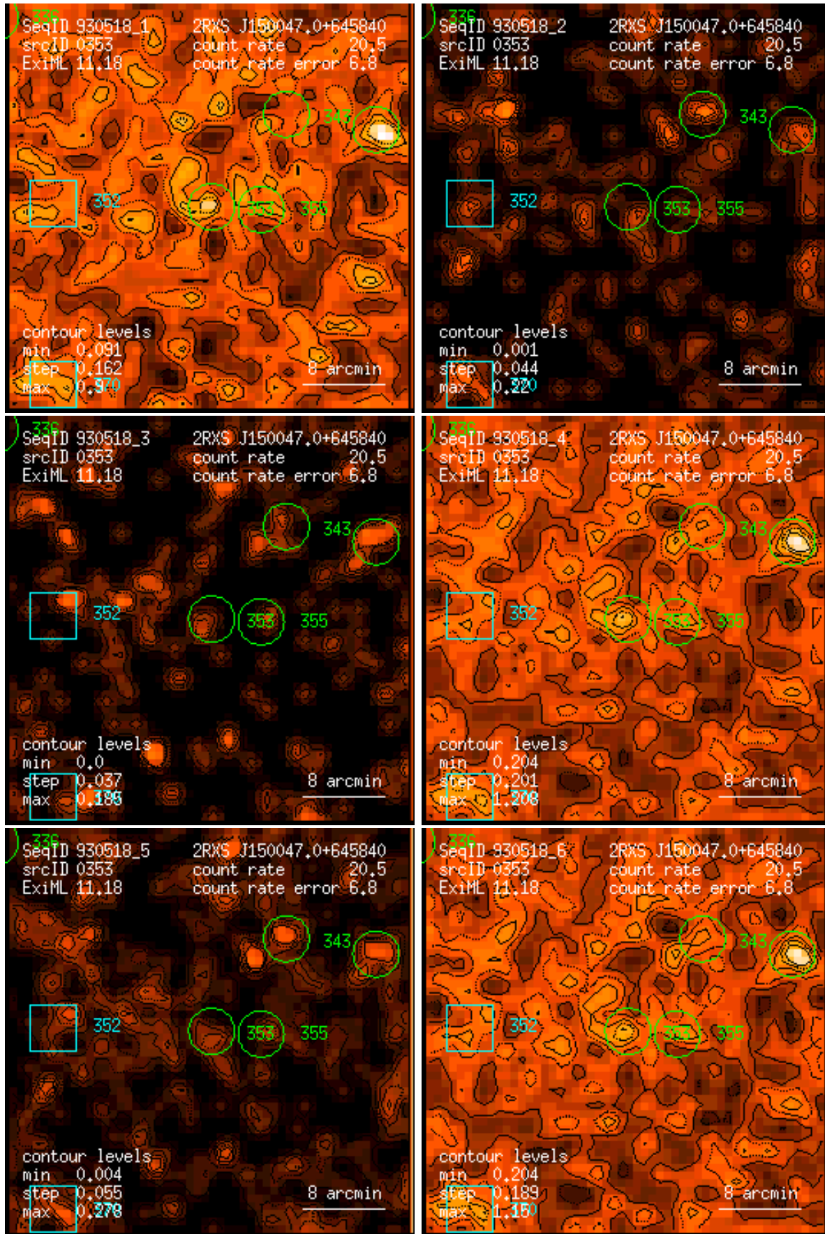
Figure 353: RASS 930518: detection 0353: band rate images, Gaussian filter: (1) PSPC channels 11 – 41, (2) 52 – 90, (3) 91 – 201, (4) 11 – 235, (5) 52 – 201, (6) 11 – 201. Broad band rates in counts/ks. Band rate contour levels in counts/ks/arcmin 2 .
