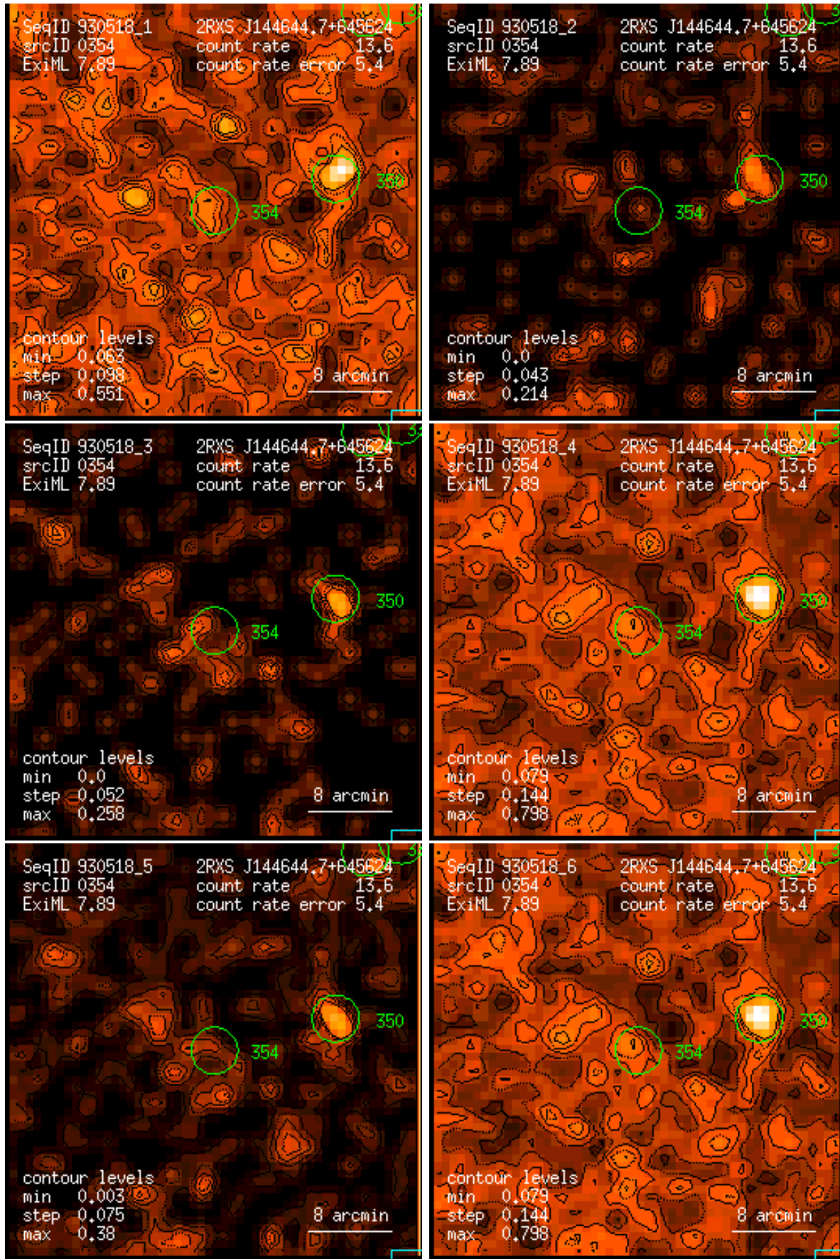
Figure 354: RASS 930518: detection 0354: band rate images, Gaussian filter: (1) PSPC channels 11 – 41, (2) 52 – 90, (3) 91 – 201, (4) 11 – 235, (5) 52 – 201, (6) 11 – 201. Broad band rates in counts/ks. Band rate contour levels in counts/ks/arcmin 2 .
