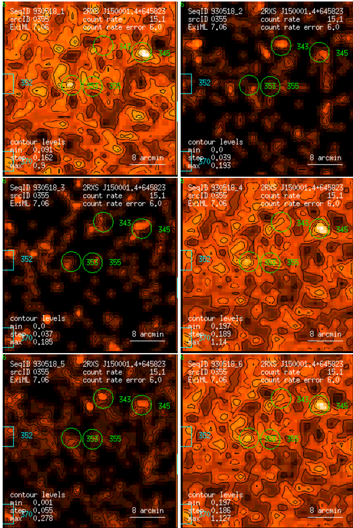
Figure 355: RASS 930518: detection 0355: band rate images, Gaussian filter: (1) PSPC channels 11 – 41, (2) 52 – 90, (3) 91 – 201, (4) 11 – 235, (5) 52 – 201, (6) 11 – 201. Broad band rates in counts/ks. Band rate contour levels in counts/ks/arcmin 2 .
