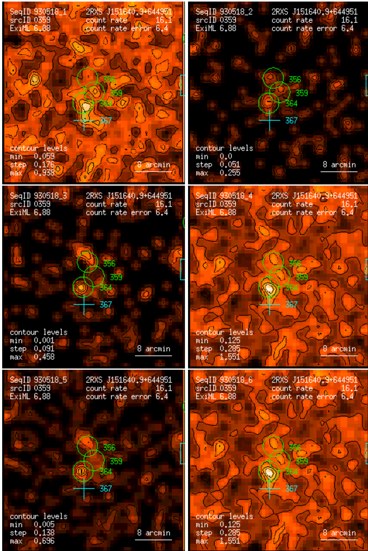
Figure 359: RASS 930518: detection 0359: band rate images, Gaussian filter: (1) PSPC channels 11 – 41, (2) 52 – 90, (3) 91 – 201, (4) 11 – 235, (5) 52 – 201, (6) 11 – 201. Broad band rates in counts/ks. Band rate contour levels in counts/ks/arcmin 2 .
