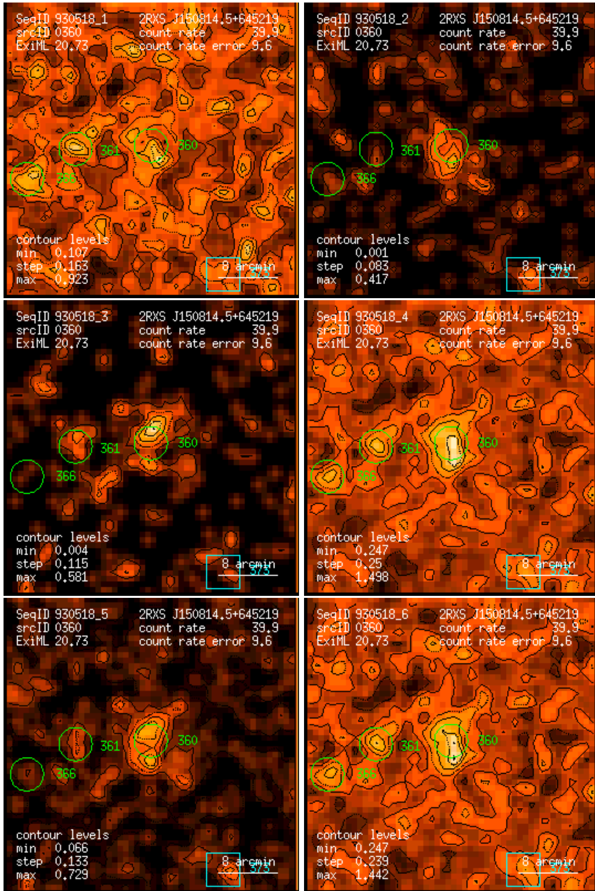
Figure 360: RASS 930518: detection 0360: band rate images, Gaussian filter: (1) PSPC channels 11 – 41, (2) 52 – 90, (3) 91 – 201, (4) 11 – 235, (5) 52 – 201, (6) 11 – 201. Broad band rates in counts/ks. Band rate contour levels in counts/ks/arcmin 2 .
