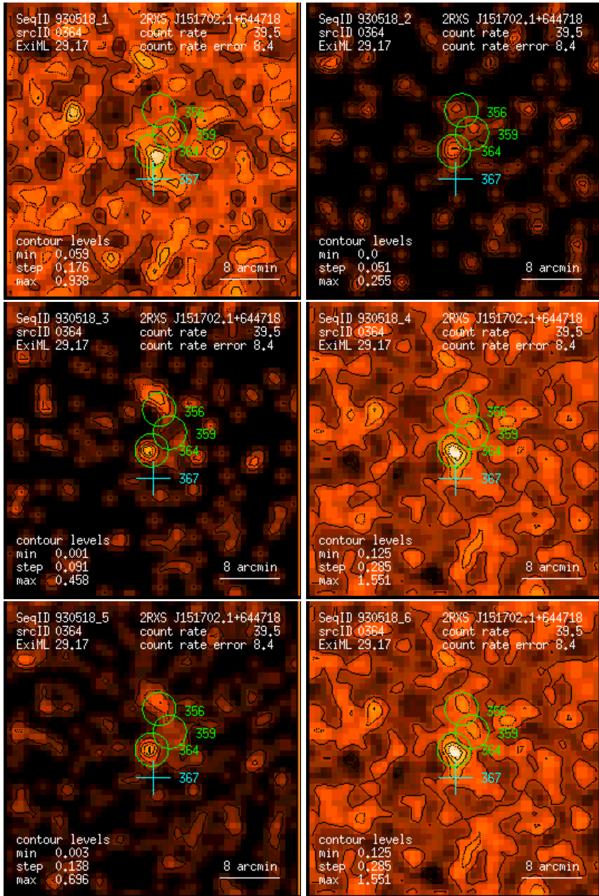
Figure 364: RASS 930518: detection 0364: band rate images, Gaussian filter: (1) PSPC channels 11 – 41, (2) 52 – 90, (3) 91 – 201, (4) 11 – 235, (5) 52 – 201, (6) 11 – 201. Broad band rates in counts/ks. Band rate contour levels in counts/ks/arcmin 2 .
