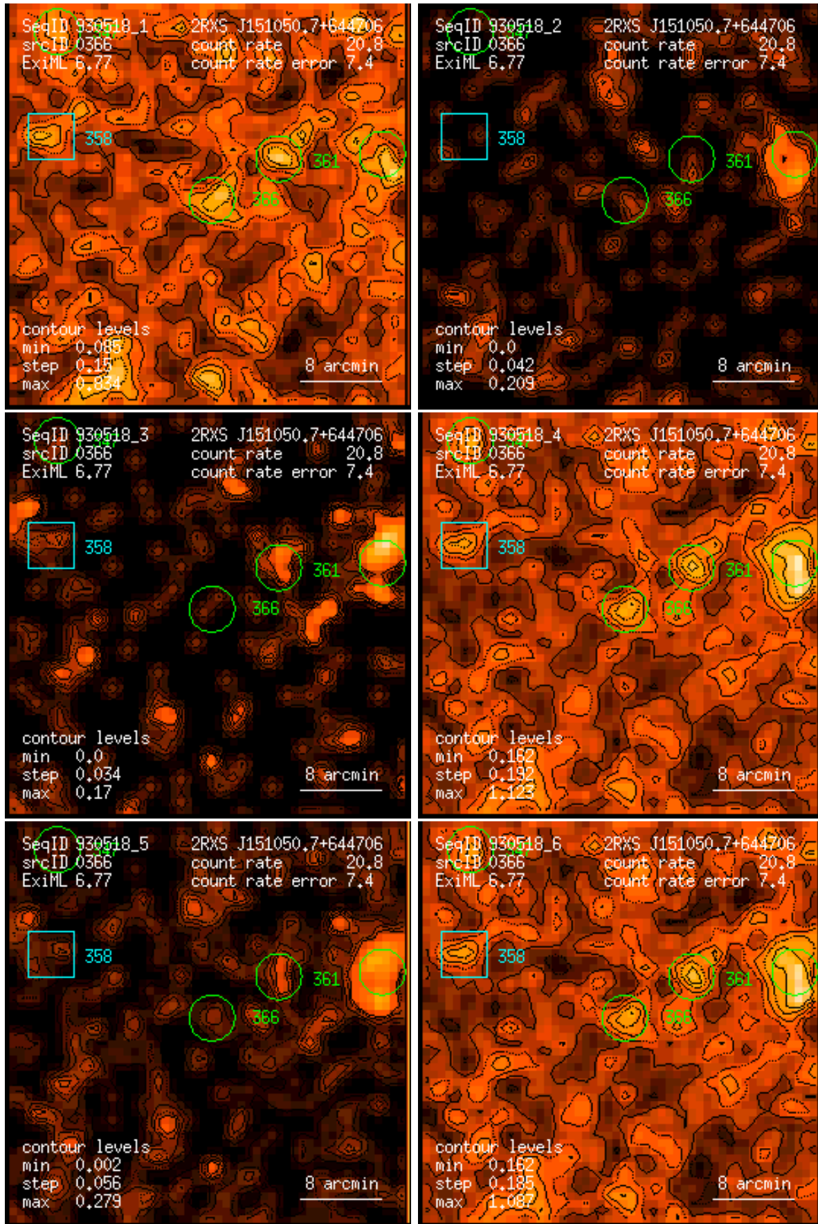
Figure 366: RASS 930518: detection 0366: band rate images, Gaussian filter: (1) PSPC channels 11 – 41, (2) 52 – 90, (3) 91 – 201, (4) 11 – 235, (5) 52 – 201, (6) 11 – 201. Broad band rates in counts/ks. Band rate contour levels in counts/ks/arcmin 2 .
