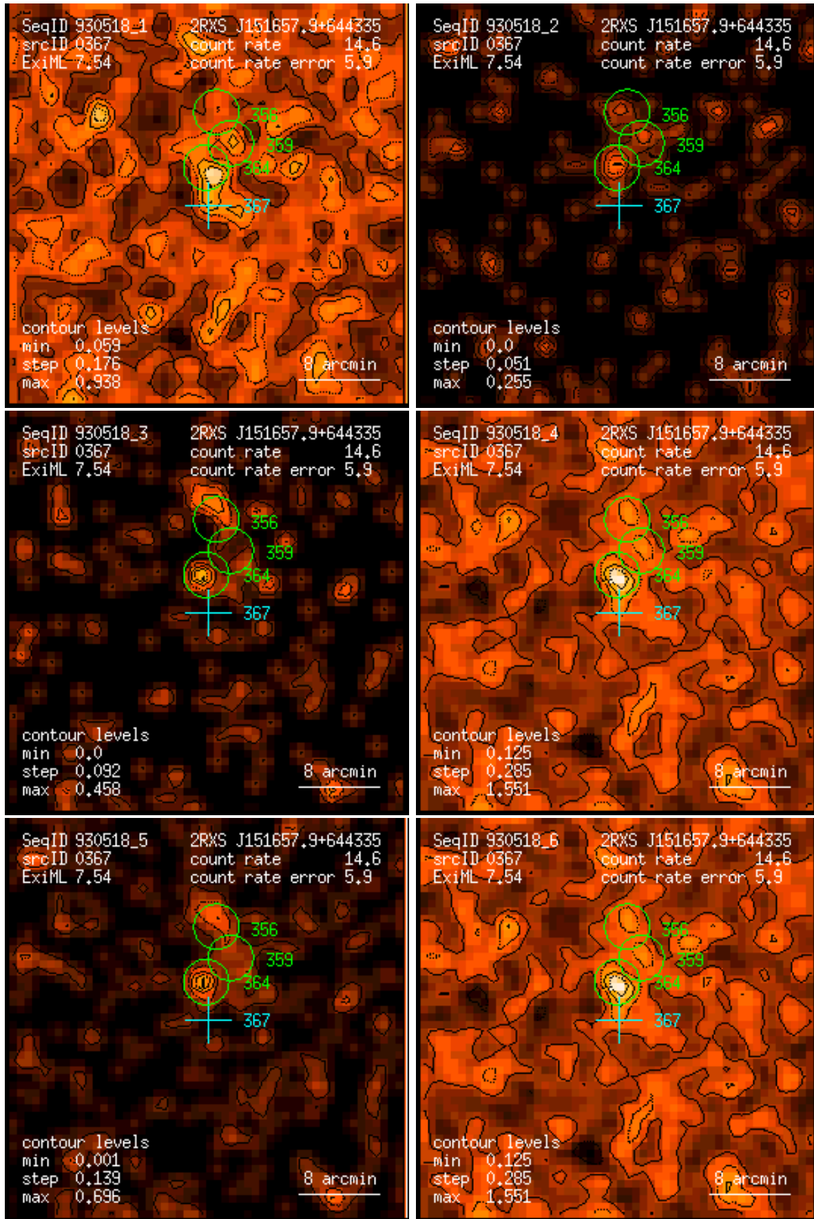
Figure 367: RASS 930518: detection 0367: band rate images, Gaussian filter: (1) PSPC channels 11 – 41, (2) 52 – 90, (3) 91 – 201, (4) 11 – 235, (5) 52 – 201, (6) 11 – 201. Broad band rates in counts/ks. Band rate contour levels in counts/ks/arcmin 2 .
