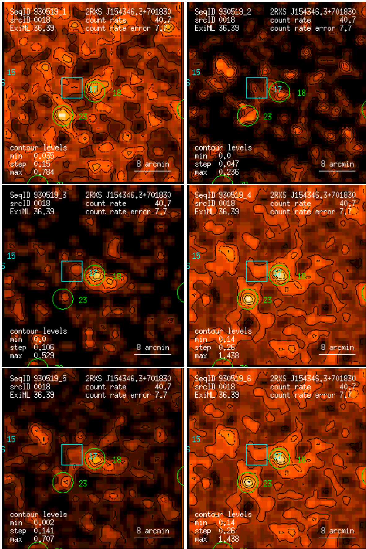
Figure 18: RASS 930519: detection 0018: band rate images, Gaussian filter: (1) PSPC channels 11 – 41, (2) 52 – 90, (3) 91 – 201, (4) 11 – 235, (5) 52 – 201, (6) 11 – 201. Broad band rates in counts/ks. Band rate contour levels in counts/ks/arcmin 2 .
