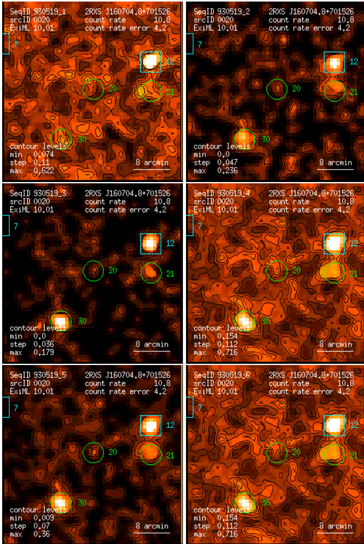
Figure 20: RASS 930519: detection 0020: band rate images, Gaussian filter: (1) PSPC channels 11 – 41, (2) 52 – 90, (3) 91 – 201, (4) 11 – 235, (5) 52 – 201, (6) 11 – 201. Broad band rates in counts/ks. Band rate contour levels in counts/ks/arcmin 2 .
