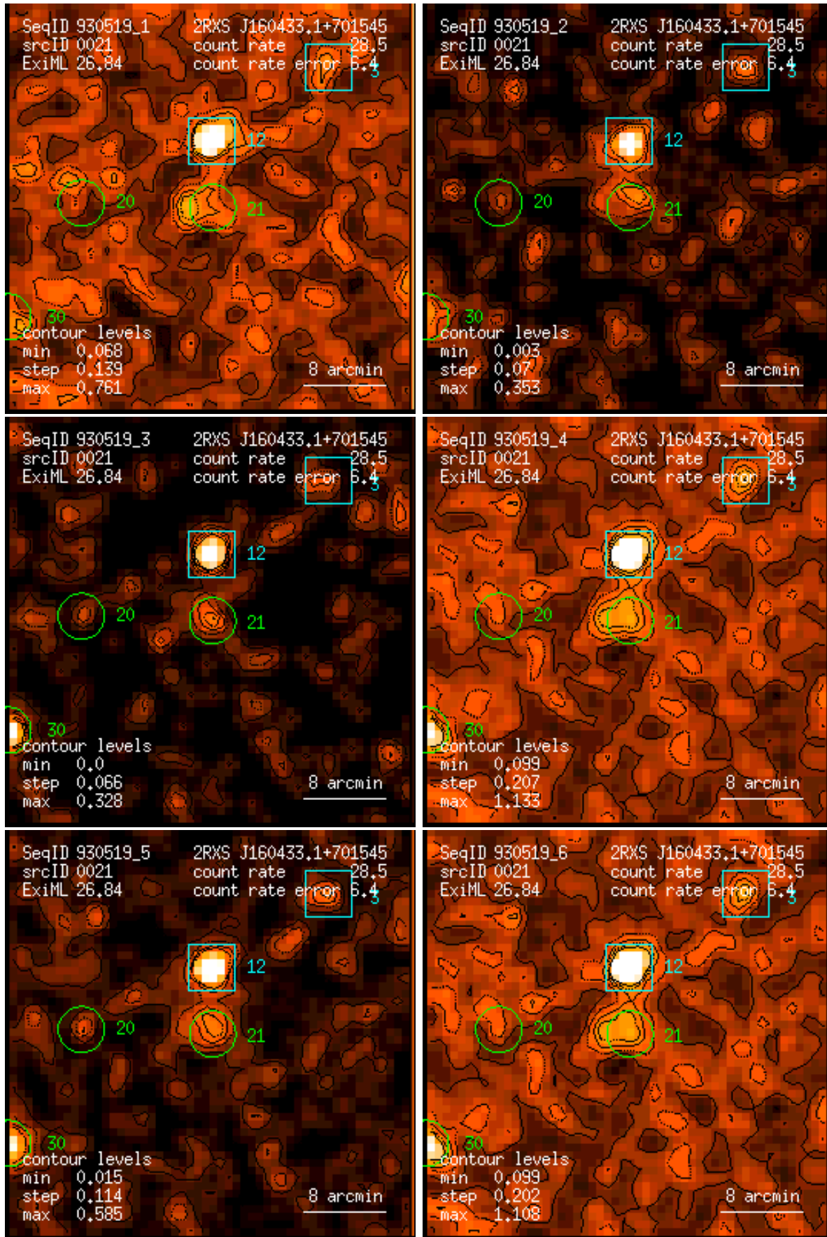
Figure 21: RASS 930519: detection 0021: band rate images, Gaussian filter: (1) PSPC channels 11 – 41, (2) 52 – 90, (3) 91 – 201, (4) 11 – 235, (5) 52 – 201, (6) 11 – 201. Broad band rates in counts/ks. Band rate contour levels in counts/ks/arcmin 2 .
