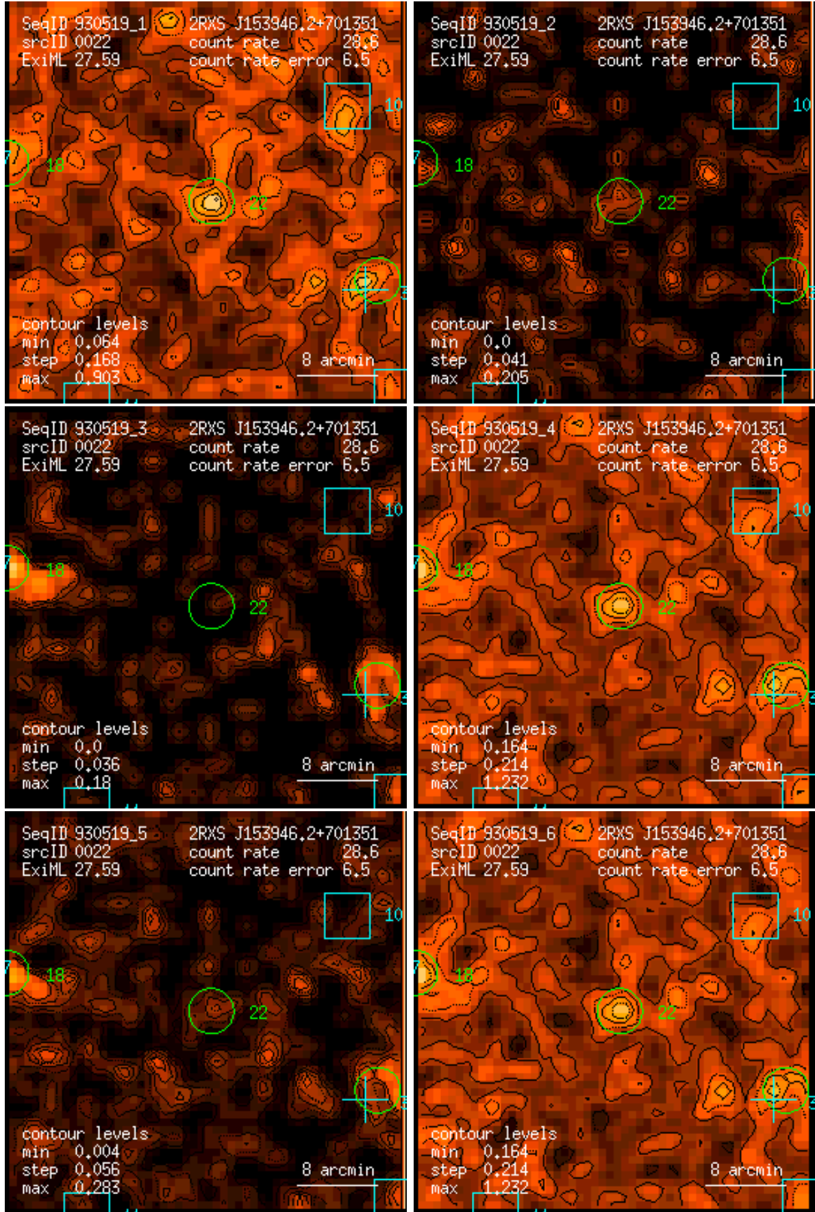
Figure 22: RASS 930519: detection 0022: band rate images, Gaussian filter: (1) PSPC channels 11 – 41, (2) 52 – 90, (3) 91 – 201, (4) 11 – 235, (5) 52 – 201, (6) 11 – 201. Broad band rates in counts/ks. Band rate contour levels in counts/ks/arcmin 2 .
