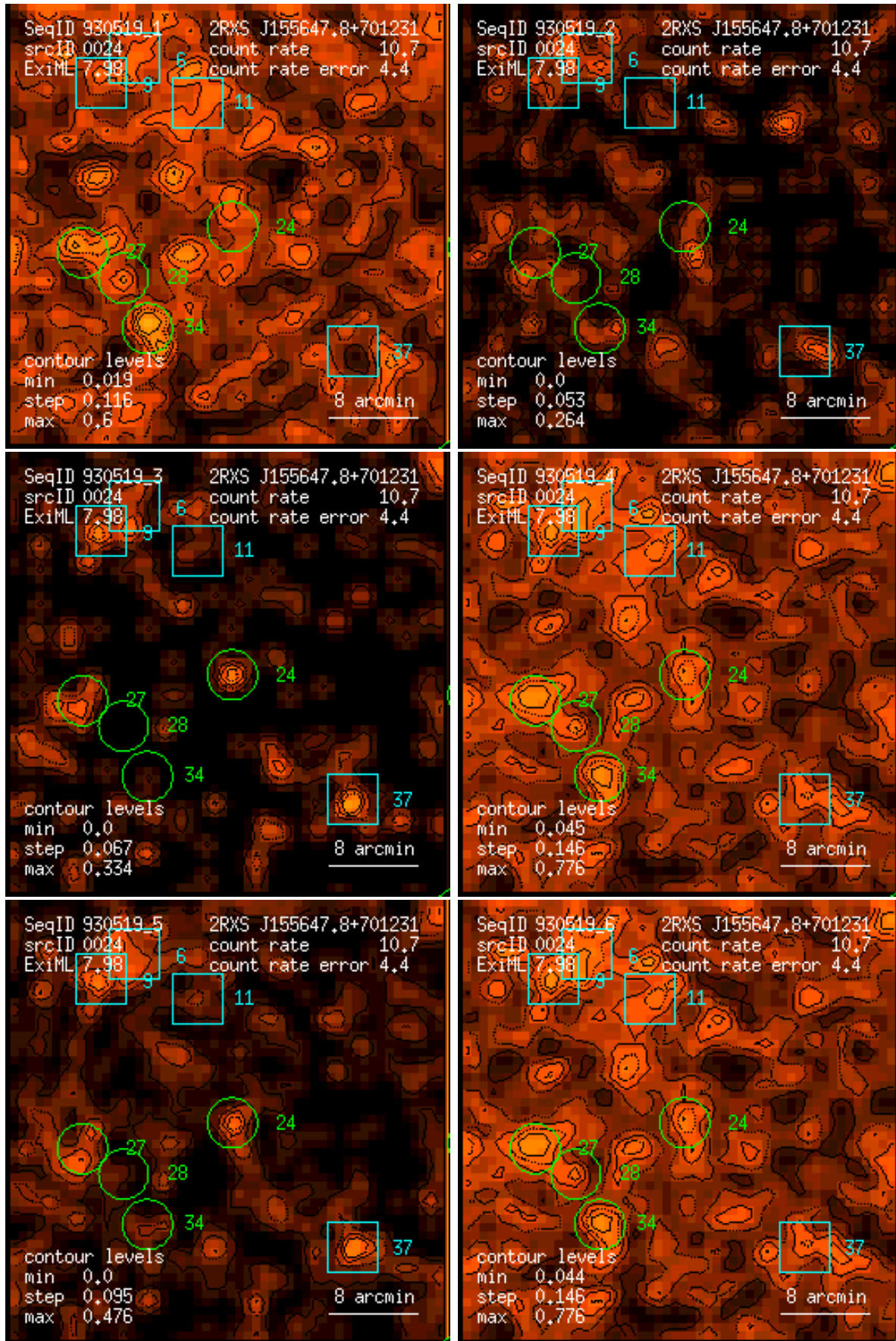
Figure 24: RASS 930519: detection 0024: band rate images, Gaussian filter: (1) PSPC channels 11 – 41, (2) 52 – 90, (3) 91 – 201, (4) 11 – 235, (5) 52 – 201, (6) 11 – 201. Broad band rates in counts/ks. Band rate contour levels in counts/ks/arcmin 2 .
