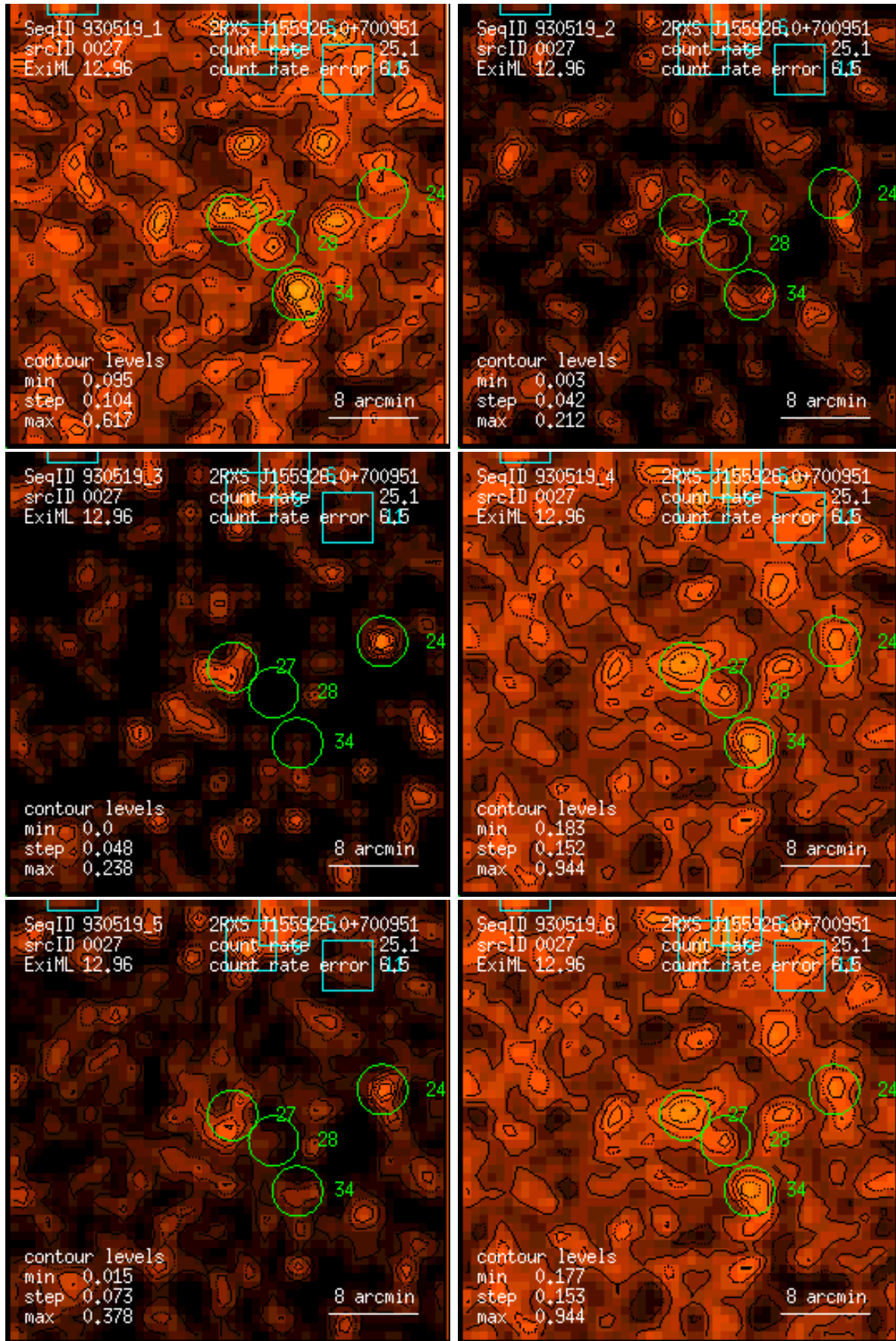
Figure 27: RASS 930519: detection 0027: band rate images, Gaussian filter: (1) PSPC channels 11 – 41, (2) 52 – 90, (3) 91 – 201, (4) 11 – 235, (5) 52 – 201, (6) 11 – 201. Broad band rates in counts/ks. Band rate contour levels in counts/ks/arcmin 2 .
