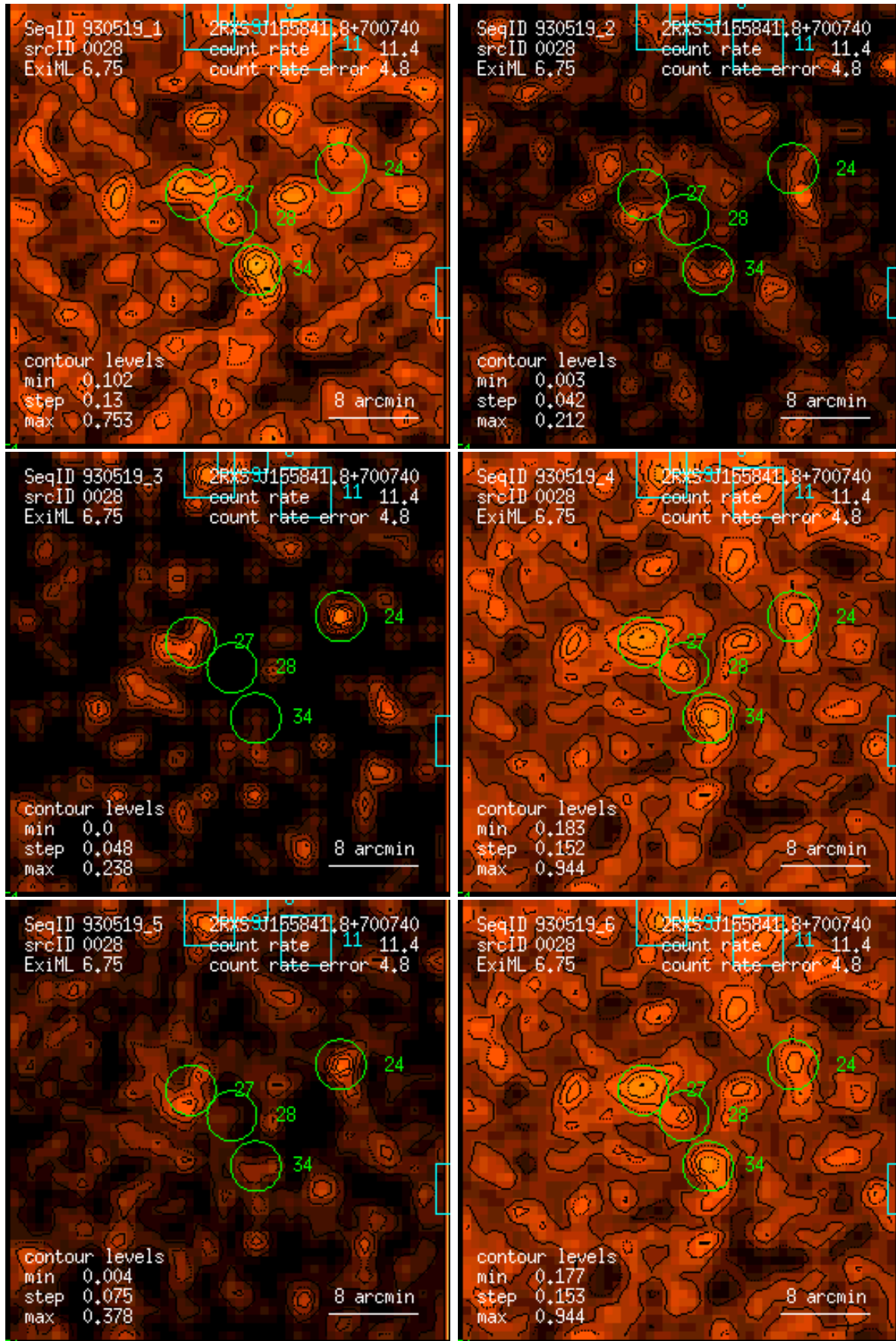
Figure 28: RASS 930519: detection 0028: band rate images, Gaussian filter: (1) PSPC channels 11 – 41, (2) 52 – 90, (3) 91 – 201, (4) 11 – 235, (5) 52 – 201, (6) 11 – 201. Broad band rates in counts/ks. Band rate contour levels in counts/ks/arcmin 2 .
