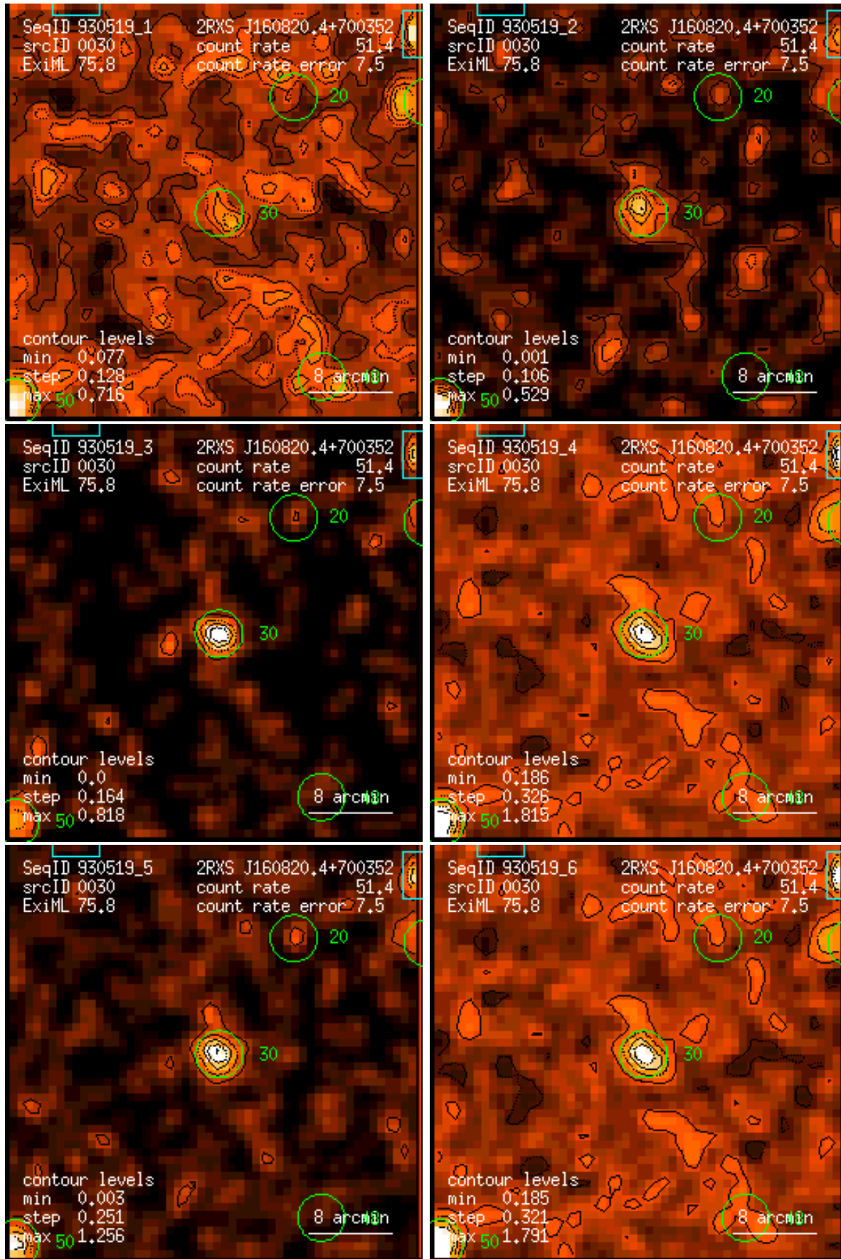
Figure 30: RASS 930519: detection 0030: band rate images, Gaussian filter: (1) PSPC channels 11 – 41, (2) 52 – 90, (3) 91 – 201, (4) 11 – 235, (5) 52 – 201, (6) 11 – 201. Broad band rates in counts/ks. Band rate contour levels in counts/ks/arcmin 2 .
