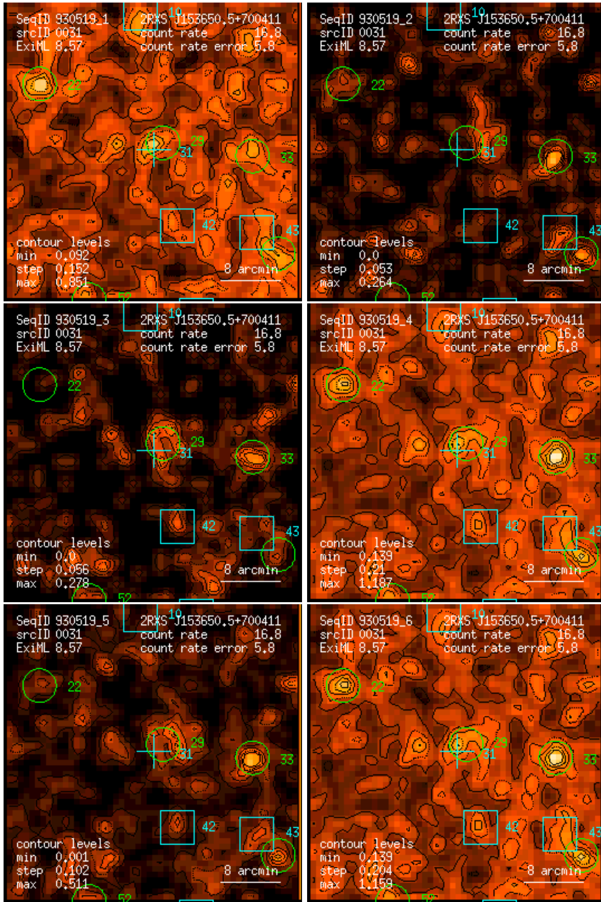
Figure 31: RASS 930519: detection 0031: band rate images, Gaussian filter: (1) PSPC channels 11 – 41, (2) 52 – 90, (3) 91 – 201, (4) 11 – 235, (5) 52 – 201, (6) 11 – 201. Broad band rates in counts/ks. Band rate contour levels in counts/ks/arcmin 2 .
