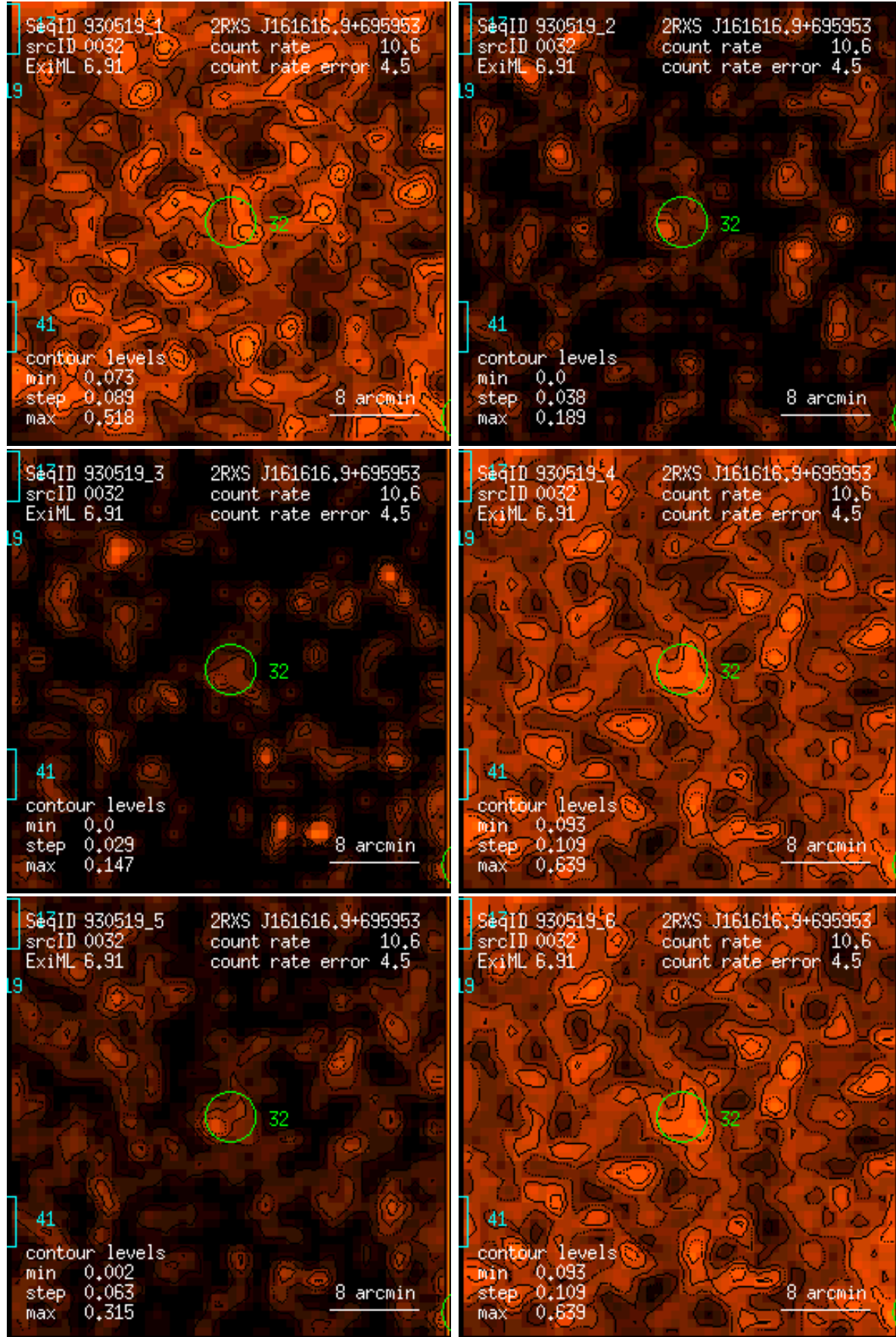
Figure 32: RASS 930519: detection 0032: band rate images, Gaussian filter: (1) PSPC channels 11 – 41, (2) 52 – 90, (3) 91 – 201, (4) 11 – 235, (5) 52 – 201, (6) 11 – 201. Broad band rates in counts/ks. Band rate contour levels in counts/ks/arcmin 2 .
