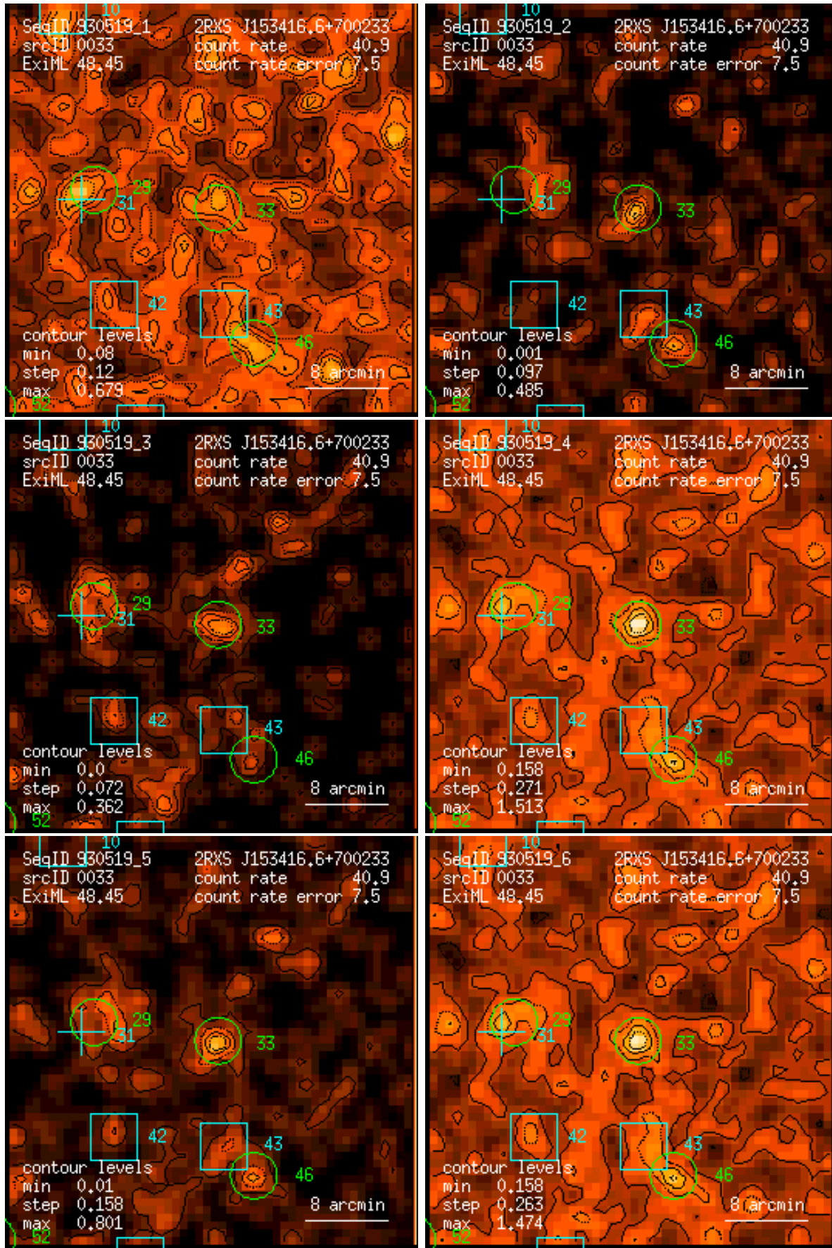
Figure 33: RASS 930519: detection 0033: band rate images, Gaussian filter: (1) PSPC channels 11 – 41, (2) 52 – 90, (3) 91 – 201, (4) 11 – 235, (5) 52 – 201, (6) 11 – 201. Broad band rates in counts/ks. Band rate contour levels in counts/ks/arcmin 2 .
