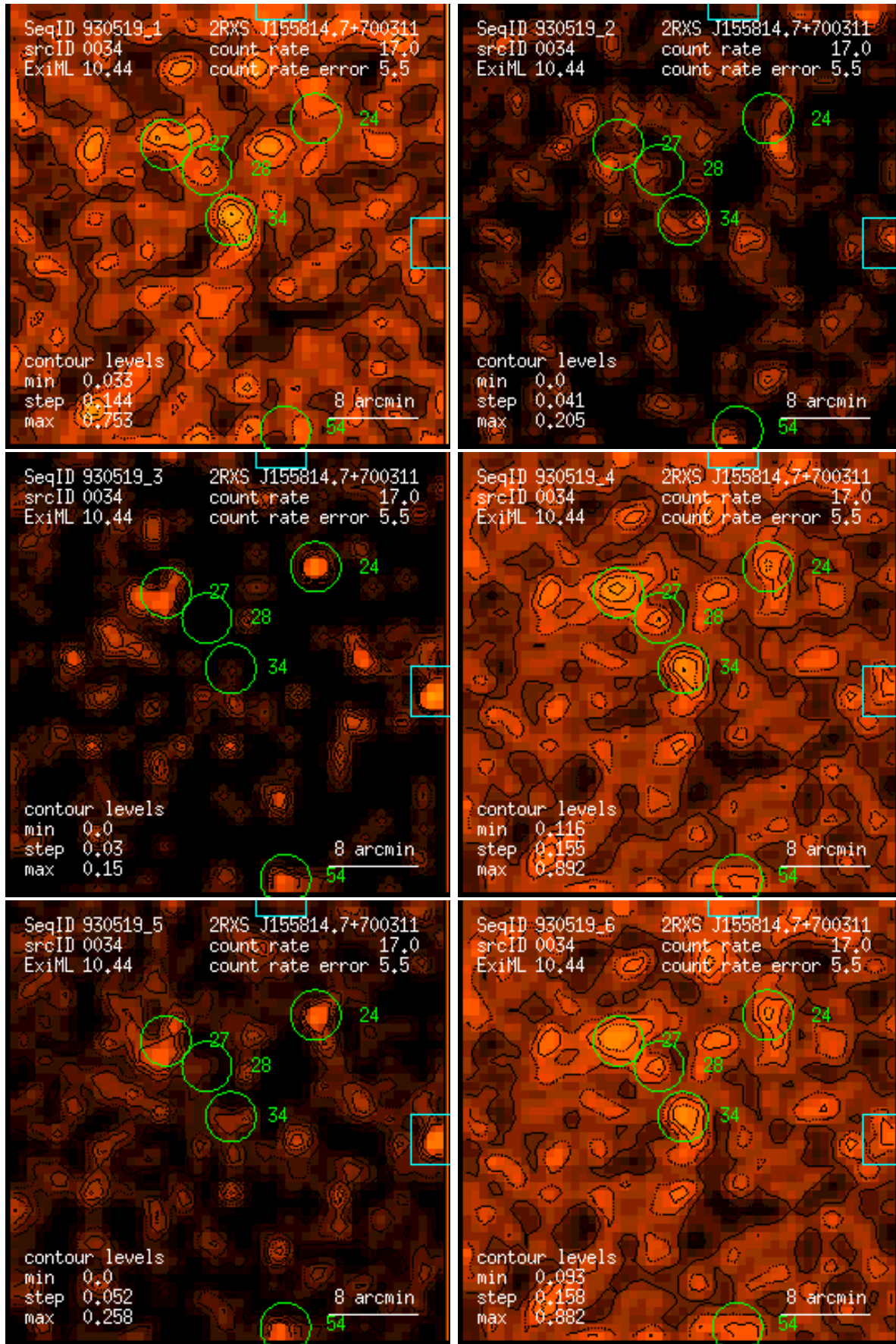
Figure 34: RASS 930519: detection 0034: band rate images, Gaussian filter: (1) PSPC channels 11 – 41, (2) 52 – 90, (3) 91 – 201, (4) 11 – 235, (5) 52 – 201, (6) 11 – 201. Broad band rates in counts/ks. Band rate contour levels in counts/ks/arcmin 2 .
