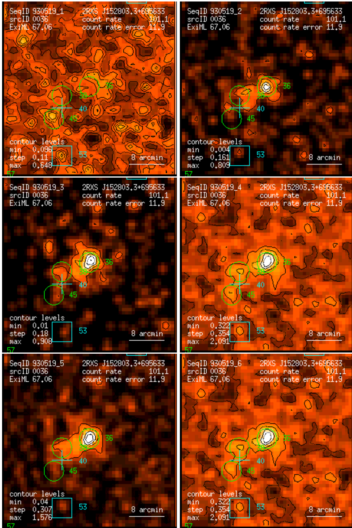
Figure 36: RASS 930519: detection 0036: band rate images, Gaussian filter: (1) PSPC channels 11 – 41, (2) 52 – 90, (3) 91 – 201, (4) 11 – 235, (5) 52 – 201, (6) 11 – 201. Broad band rates in counts/ks. Band rate contour levels in counts/ks/arcmin 2 .
