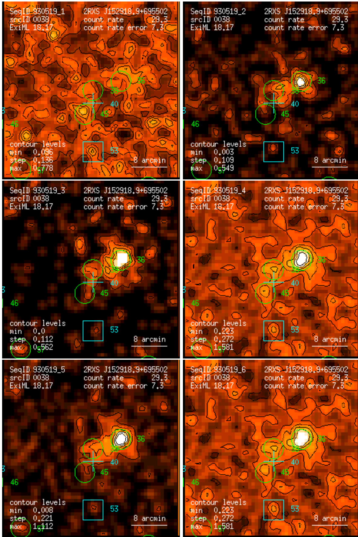
Figure 38: RASS 930519: detection 0038: band rate images, Gaussian filter: (1) PSPC channels 11 – 41, (2) 52 – 90, (3) 91 – 201, (4) 11 – 235, (5) 52 – 201, (6) 11 – 201. Broad band rates in counts/ks. Band rate contour levels in counts/ks/arcmin 2 .
