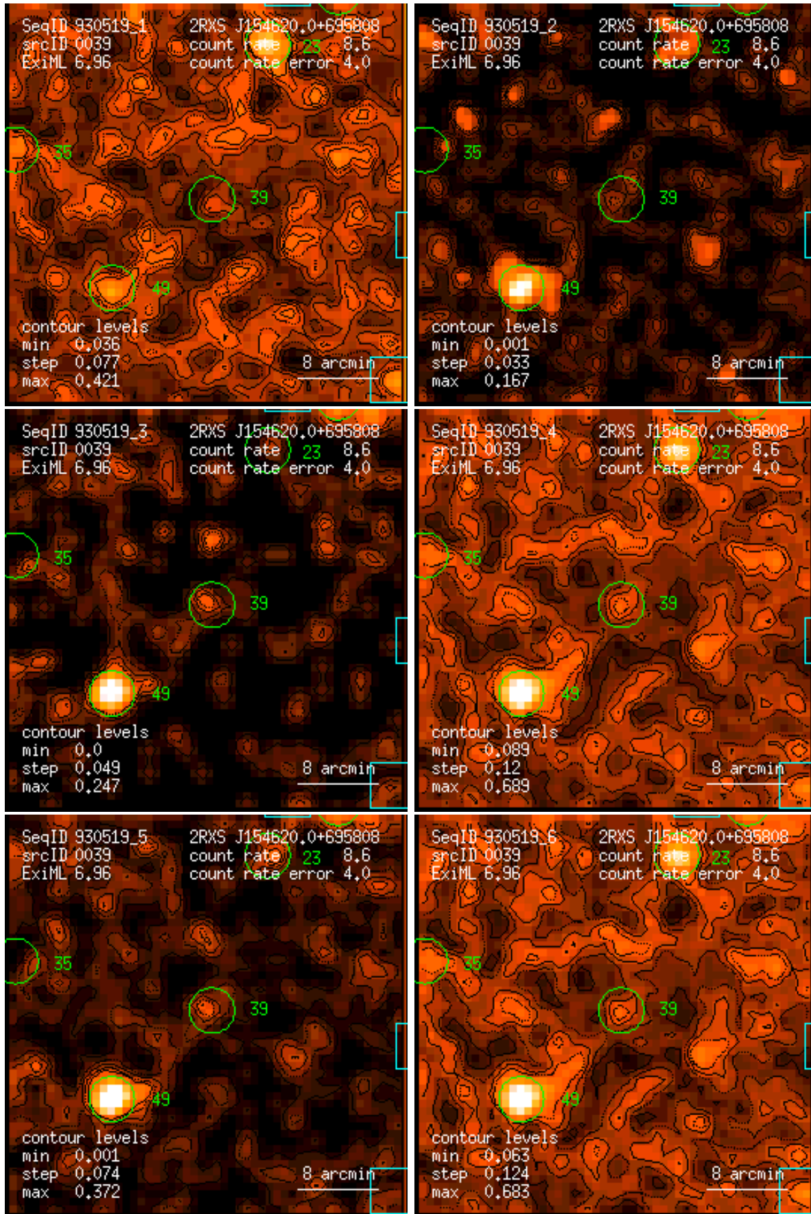
Figure 39: RASS 930519: detection 0039: band rate images, Gaussian filter: (1) PSPC channels 11 – 41, (2) 52 – 90, (3) 91 – 201, (4) 11 – 235, (5) 52 – 201, (6) 11 – 201. Broad band rates in counts/ks. Band rate contour levels in counts/ks/arcmin 2 .
