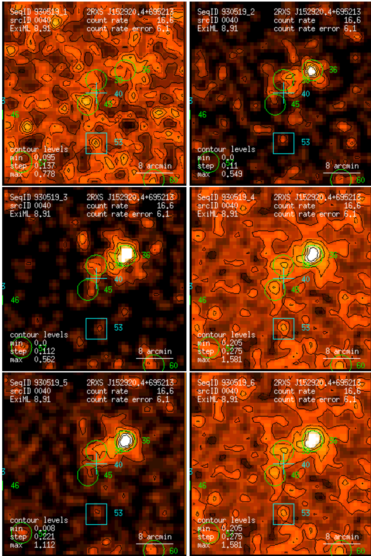
Figure 40: RASS 930519: detection 0040: band rate images, Gaussian filter: (1) PSPC channels 11 – 41, (2) 52 – 90, (3) 91 – 201, (4) 11 – 235, (5) 52 – 201, (6) 11 – 201. Broad band rates in counts/ks. Band rate contour levels in counts/ks/arcmin 2 .
