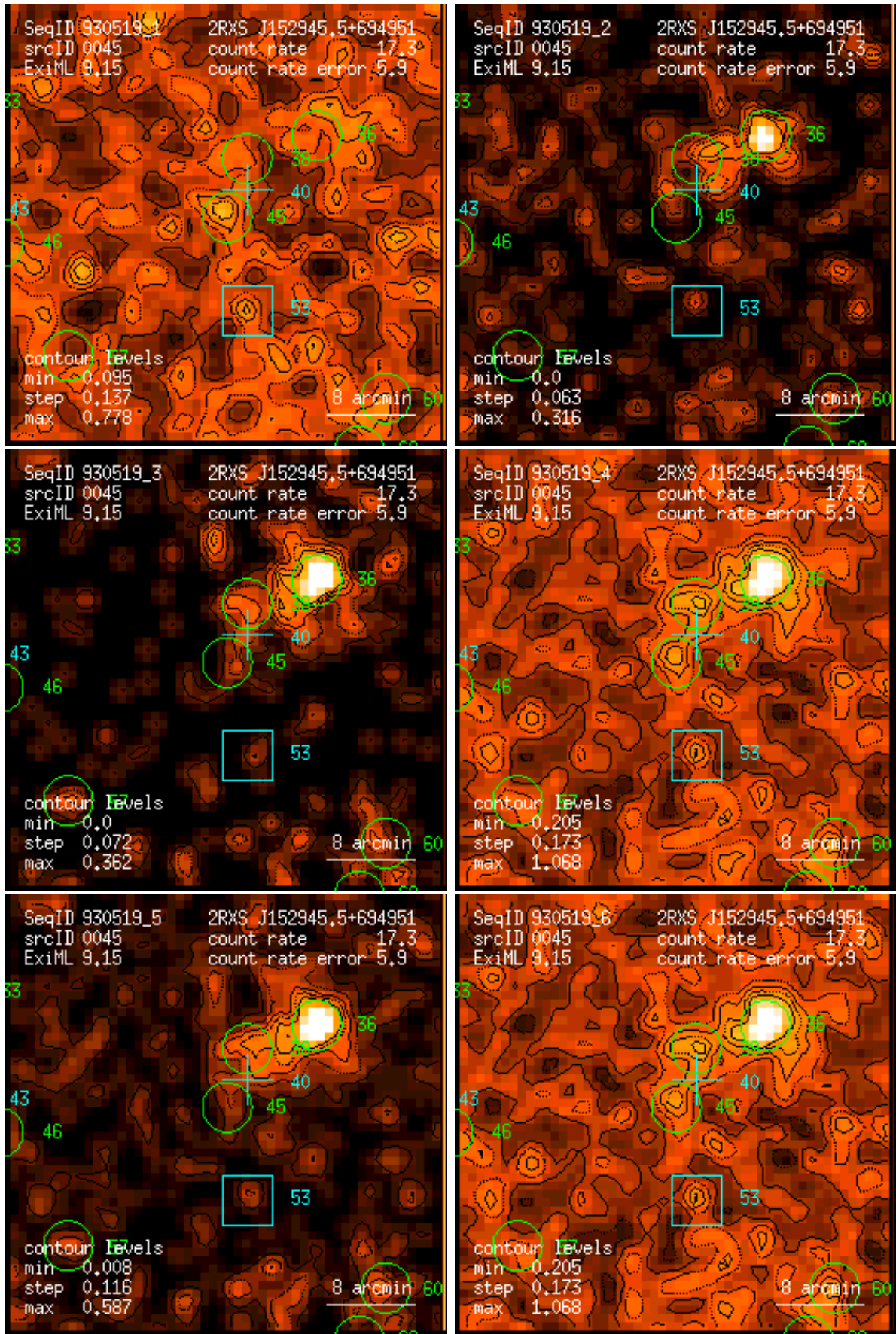
Figure 45: RASS 930519: detection 0045: band rate images, Gaussian filter: (1) PSPC channels 11 – 41, (2) 52 – 90, (3) 91 – 201, (4) 11 – 235, (5) 52 – 201, (6) 11 – 201. Broad band rates in counts/ks. Band rate contour levels in counts/ks/arcmin 2 .
