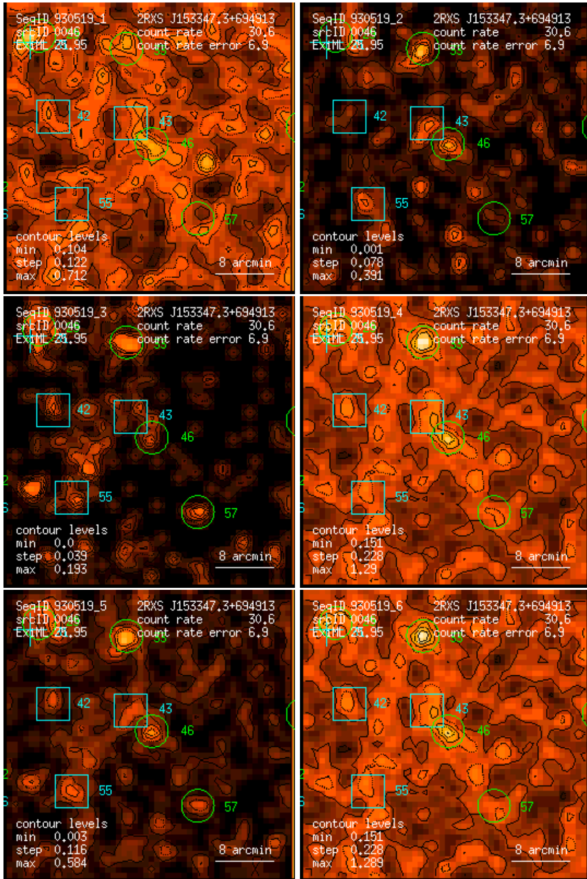
Figure 46: RASS 930519: detection 0046: band rate images, Gaussian filter: (1) PSPC channels 11 – 41, (2) 52 – 90, (3) 91 – 201, (4) 11 – 235, (5) 52 – 201, (6) 11 – 201. Broad band rates in counts/ks. Band rate contour levels in counts/ks/arcmin 2 .
