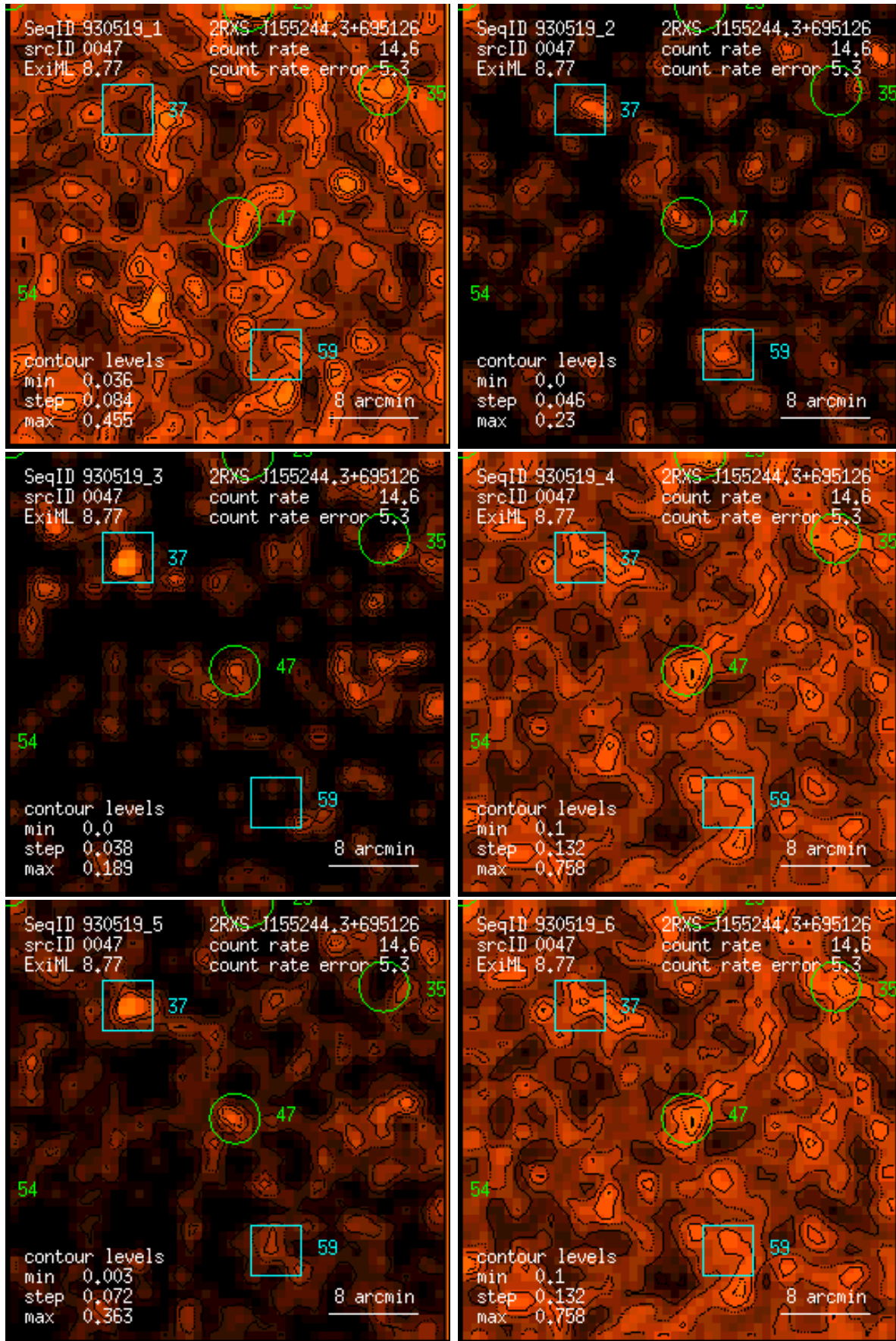
Figure 47: RASS 930519: detection 0047: band rate images, Gaussian filter: (1) PSPC channels 11 – 41, (2) 52 – 90, (3) 91 – 201, (4) 11 – 235, (5) 52 – 201, (6) 11 – 201. Broad band rates in counts/ks. Band rate contour levels in counts/ks/arcmin 2 .
