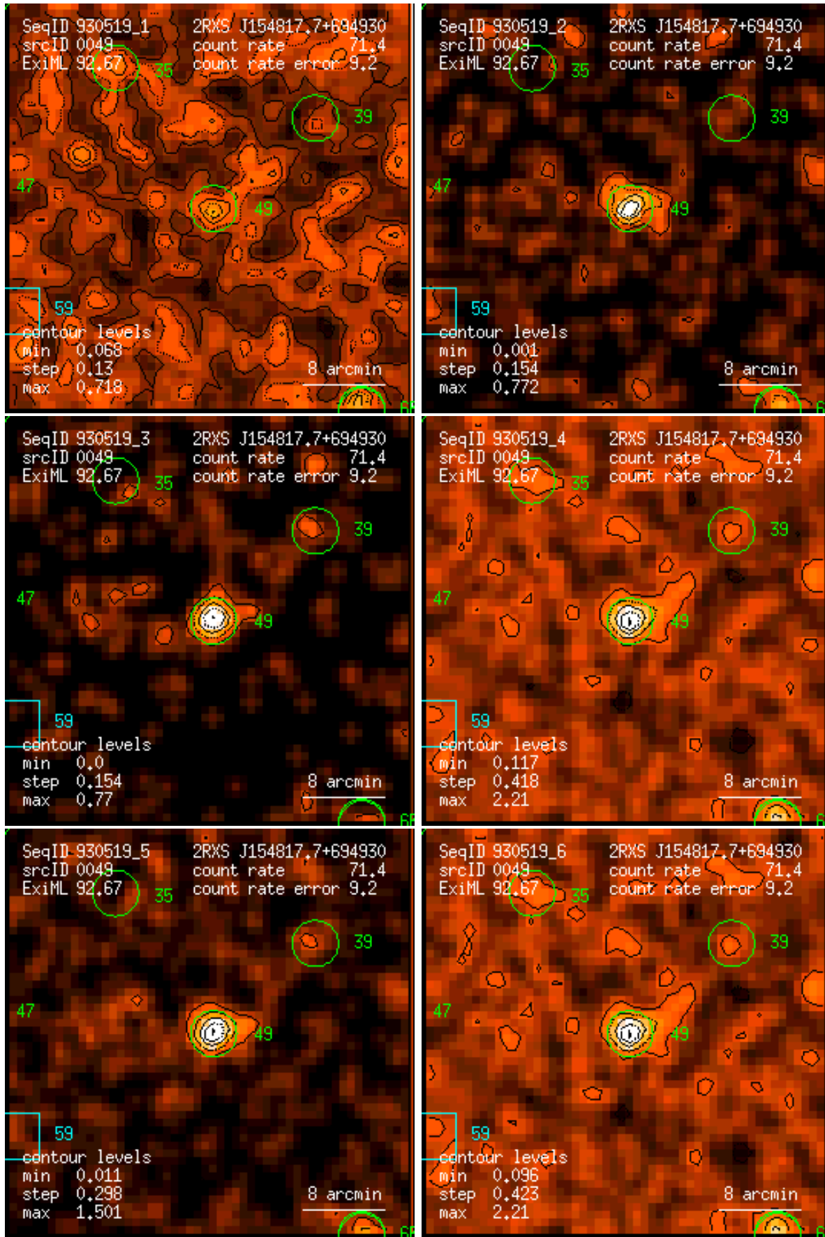
Figure 49: RASS 930519: detection 0049: band rate images, Gaussian filter: (1) PSPC channels 11 – 41, (2) 52 – 90, (3) 91 – 201, (4) 11 – 235, (5) 52 – 201, (6) 11 – 201. Broad band rates in counts/ks. Band rate contour levels in counts/ks/arcmin 2 .
