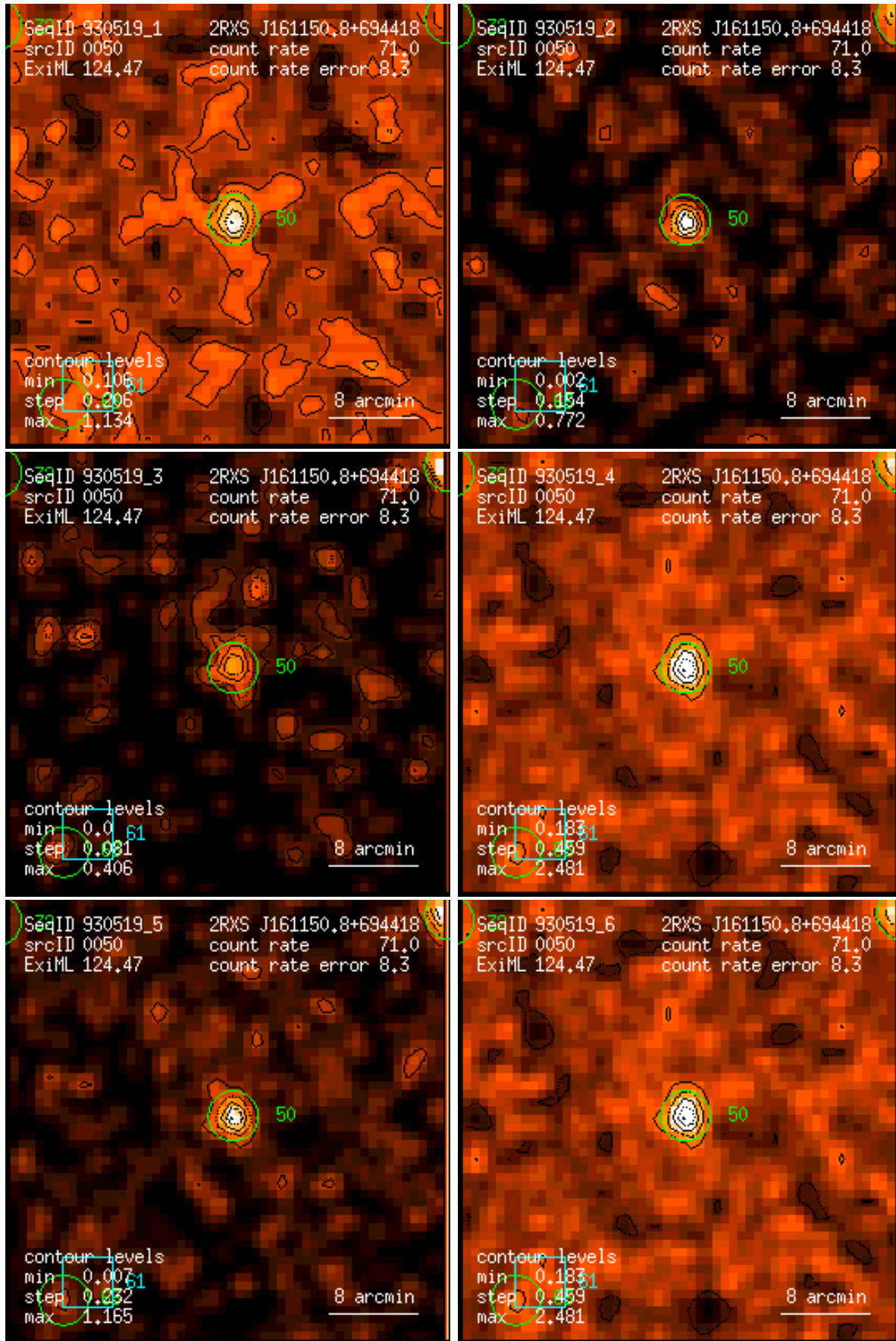
Figure 50: RASS 930519: detection 0050: band rate images, Gaussian filter: (1) PSPC channels 11 – 41, (2) 52 – 90, (3) 91 – 201, (4) 11 – 235, (5) 52 – 201, (6) 11 – 201. Broad band rates in counts/ks. Band rate contour levels in counts/ks/arcmin 2 .
