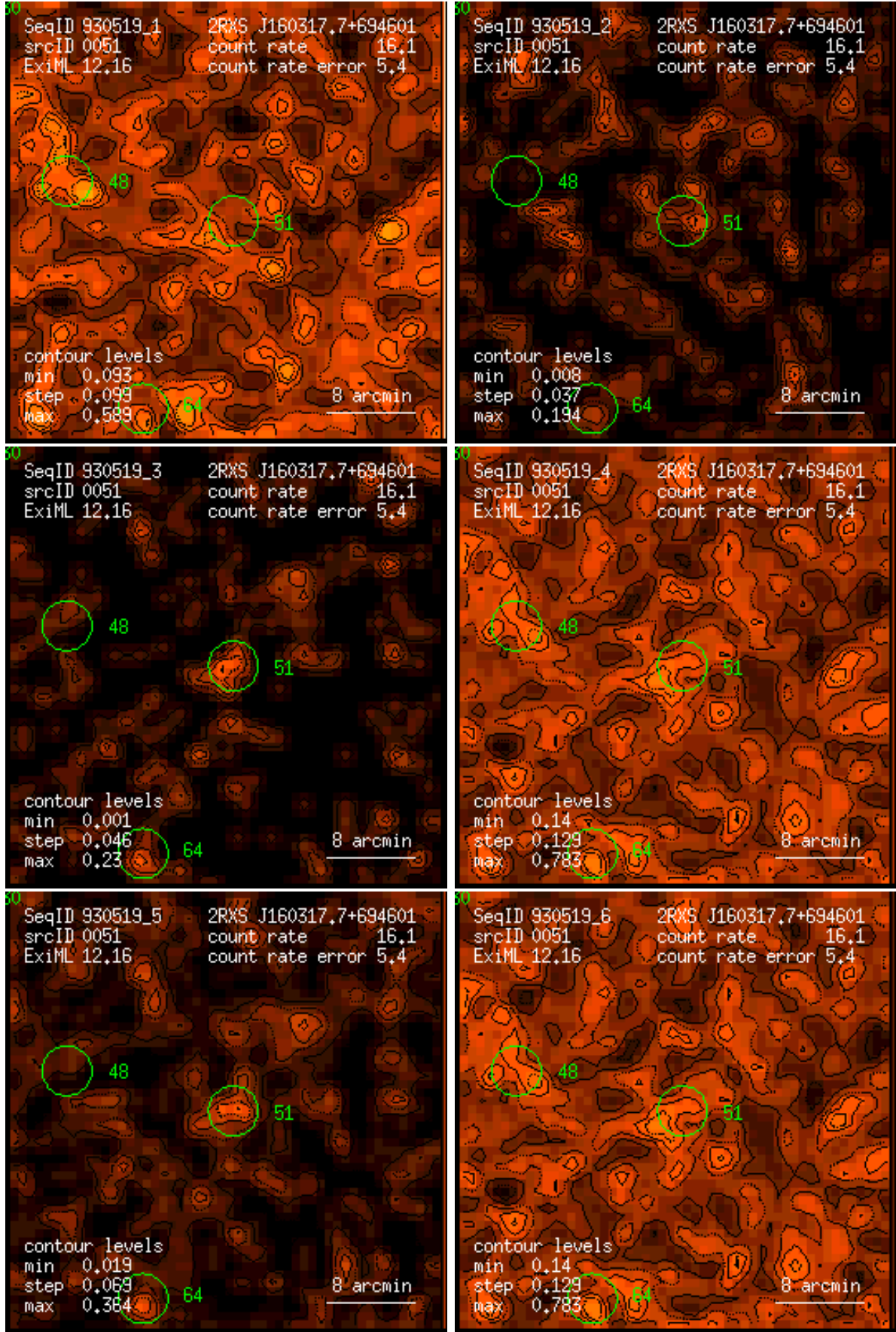
Figure 51: RASS 930519: detection 0051: band rate images, Gaussian filter: (1) PSPC channels 11 – 41, (2) 52 – 90, (3) 91 – 201, (4) 11 – 235, (5) 52 – 201, (6) 11 – 201. Broad band rates in counts/ks. Band rate contour levels in counts/ks/arcmin 2 .
