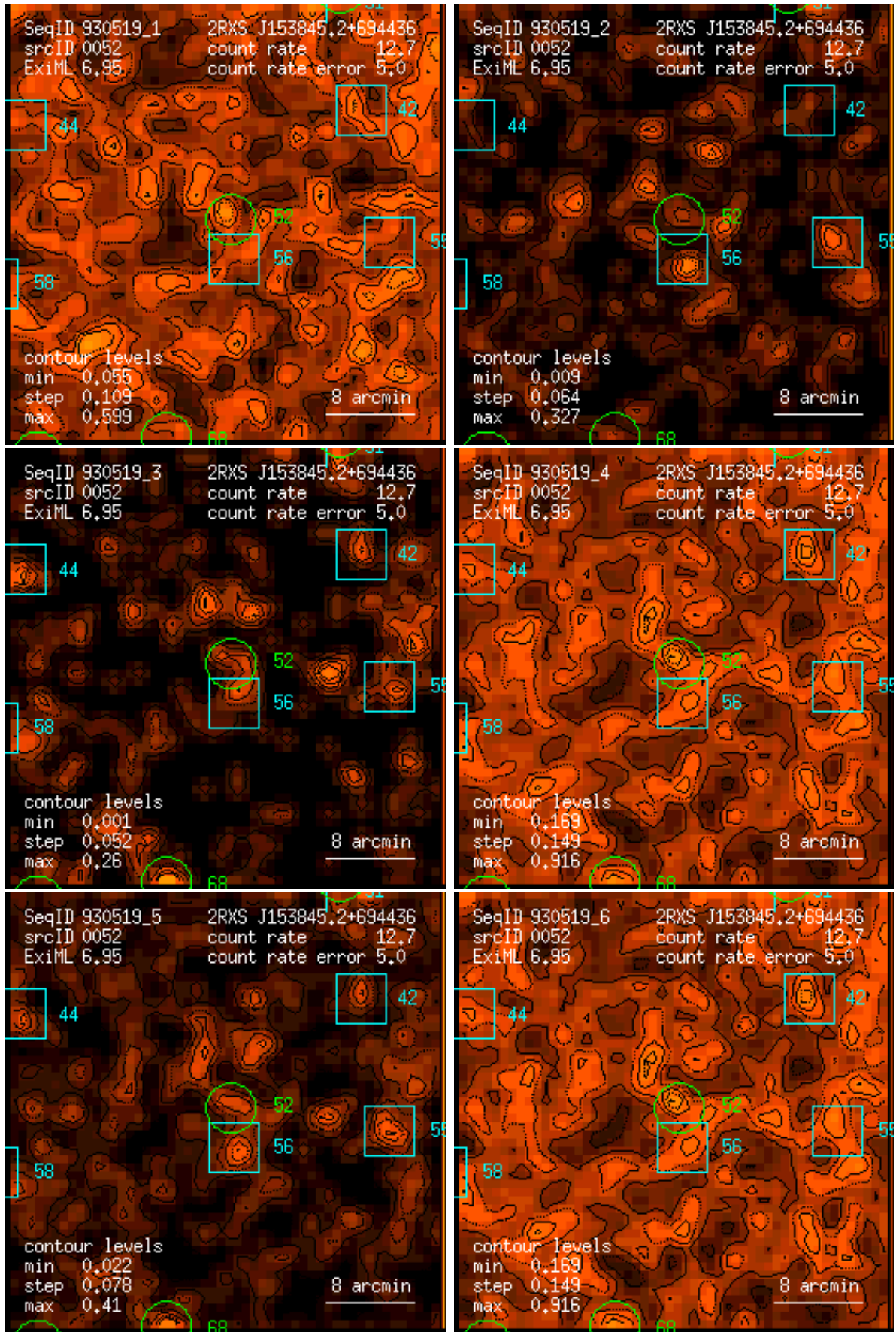
Figure 52: RASS 930519: detection 0052: band rate images, Gaussian filter: (1) PSPC channels 11 – 41, (2) 52 – 90, (3) 91 – 201, (4) 11 – 235, (5) 52 – 201, (6) 11 – 201. Broad band rates in counts/ks. Band rate contour levels in counts/ks/arcmin 2 .
